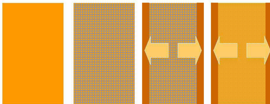
Figure 4-7a. —Four steps in the formation of Type I mottles where Fe oxides become concentrated along a ped surface: (1) the initial condition; (2) saturation of the ped and the development of reducing conditions throughout the interior of the ped; (3) drying that causes soil water to move toward the ped face, carrying soluble Fe(II) that then oxidizes to Fe(III); and (4) the final condition with Type I mottles formed at the ped face. (Diagram by M.C. Rabenhorst)
