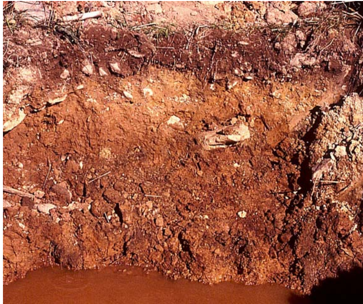
Figure 10-1.—A hydric soil formed in red parent material that meets Field Indicator TF2 (Red Parent Material) but does not have the typical gray matrix that would meet Field Indicator F3 (Depleted Matrix).
