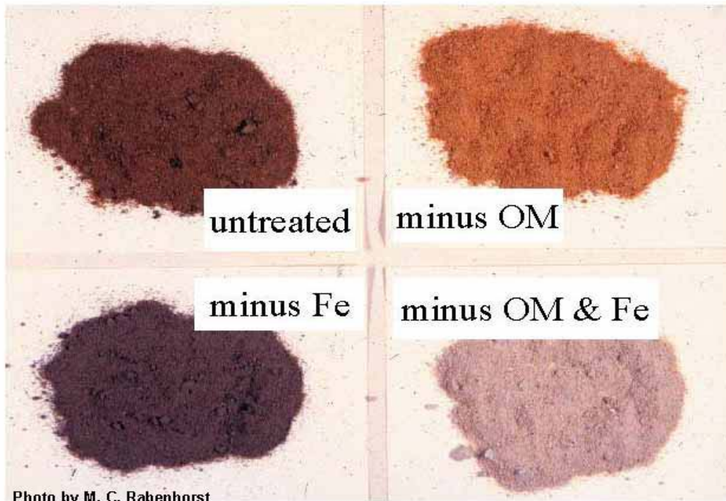
Figure 4-2. —The contributions of organic matter and iron oxides to soil color are evident in this soil sample of an Ap horizon from which organic matter and iron oxides have been removed.
