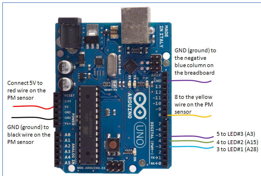
Figure 6. Schematic of wiring the Arduino board to the PM sensor and breadboard
