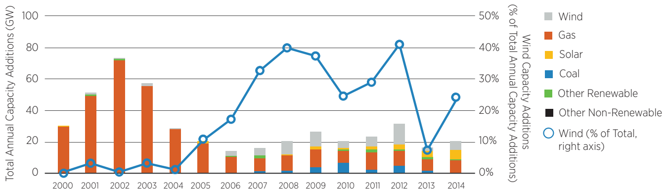
Wind Represented 24% of U.S. Electric-Generating Capacity Additions in 2014
