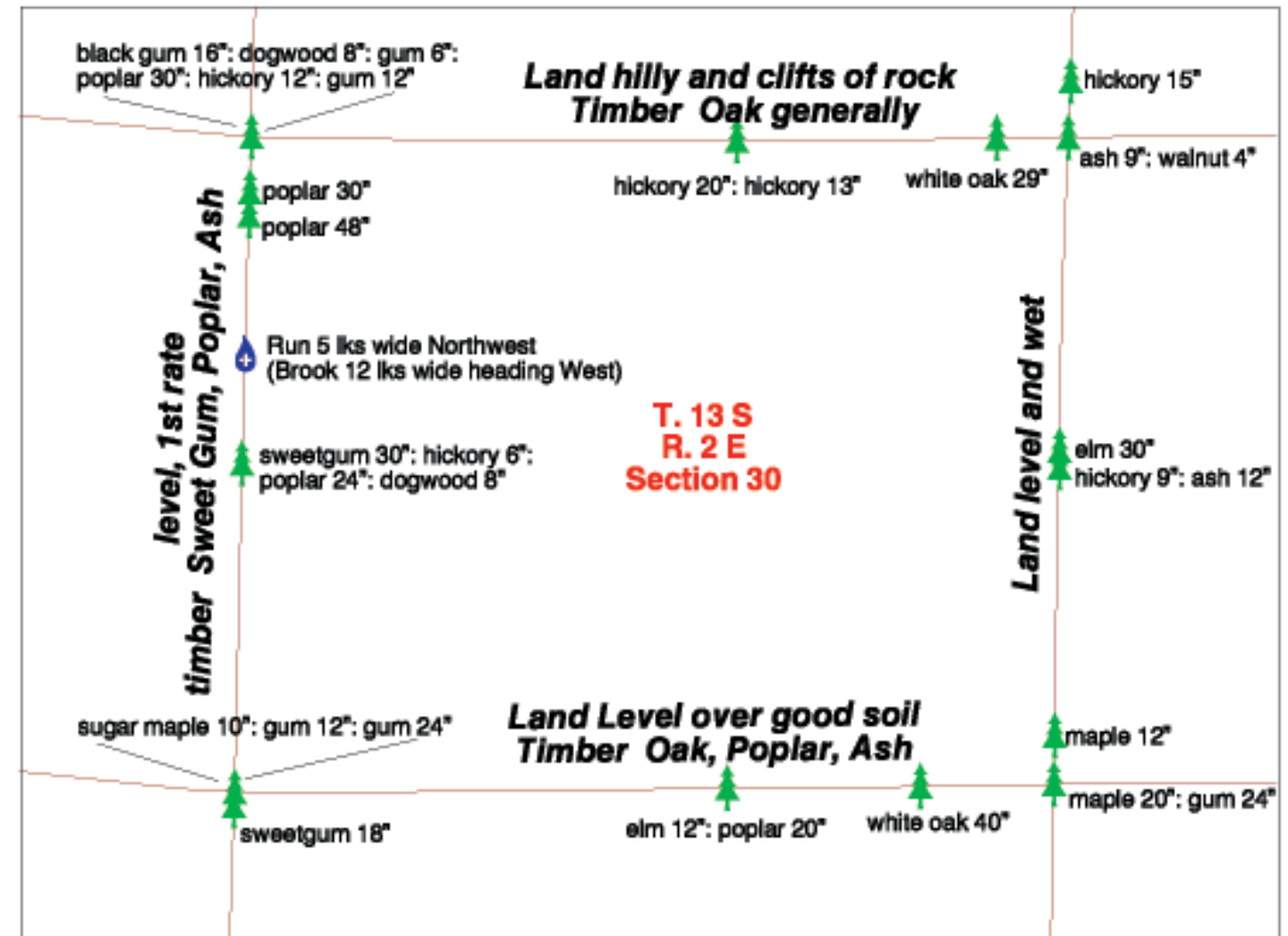
These are the 1807 Public Land Survey Notes for one section (T. 13 S., R. 2 E., Section 30) in the Cypress Quadrangle mapped at 1:24,000. The large, bold, print indicates general notes along the section lines. Tree species and basal diameter were noted along with any hydrologic features that occurred along the section line.
