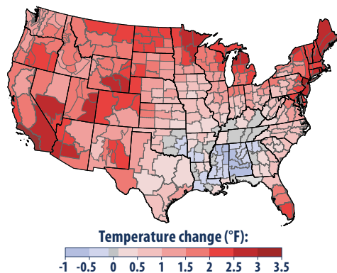
Rising temperatures in the last century. Maine has warmed twice as much as the rest of the contiguous 48 states. Source: EPA, Climate Change Indicators in the United States .
