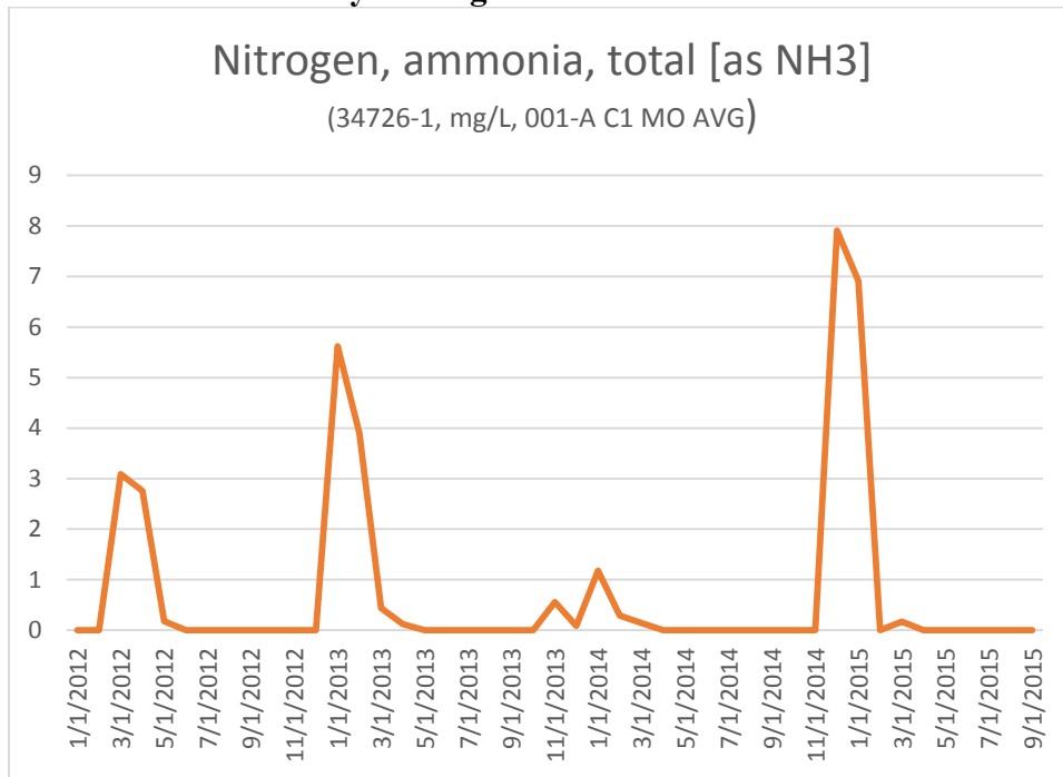
Figure 7 Exceedances of Monthly Average concentration limit for Total Ammonia
