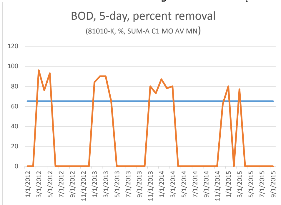
Figure 3 Violation of BOD 5 Percentage Removal Efficiency
