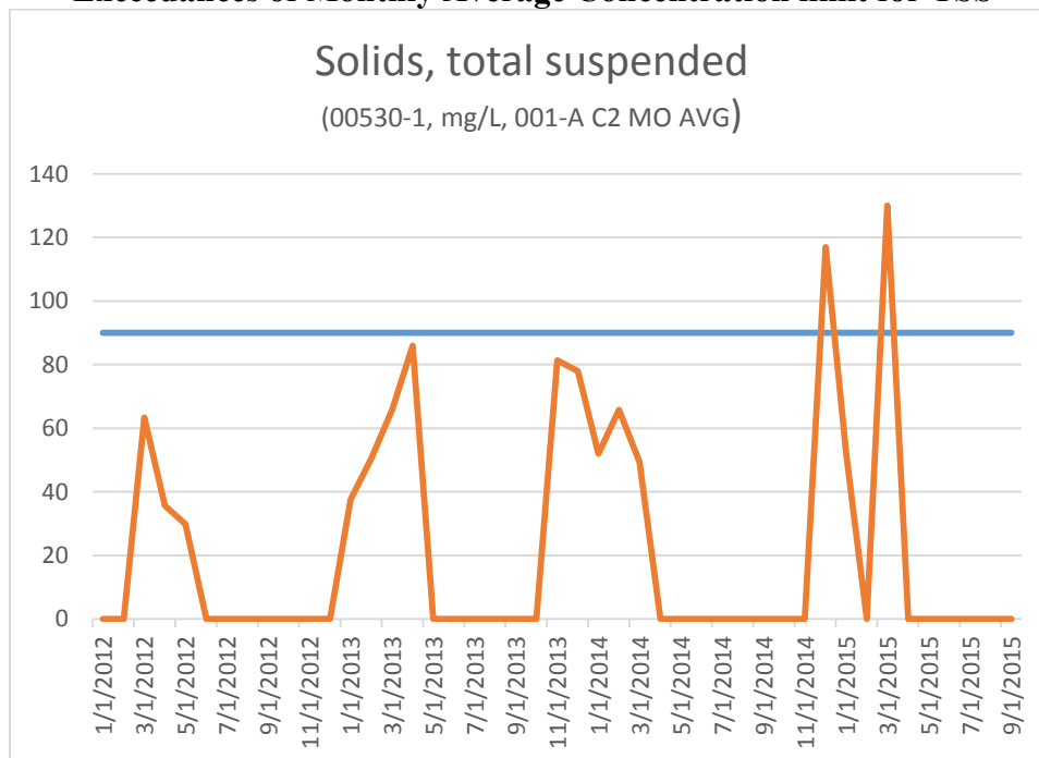
Figure 4 Exceedances of Monthly Average Concentration limit for TSS
