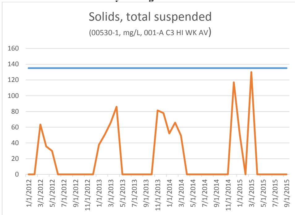
Figure 5 Exceedances of Weekly Average Concentration limit for TSS
