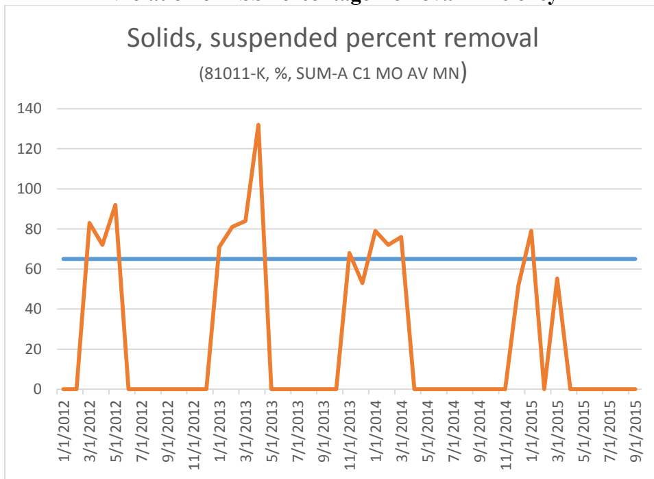
Figure 6 Violation of TSS Percentage Removal Efficiency
