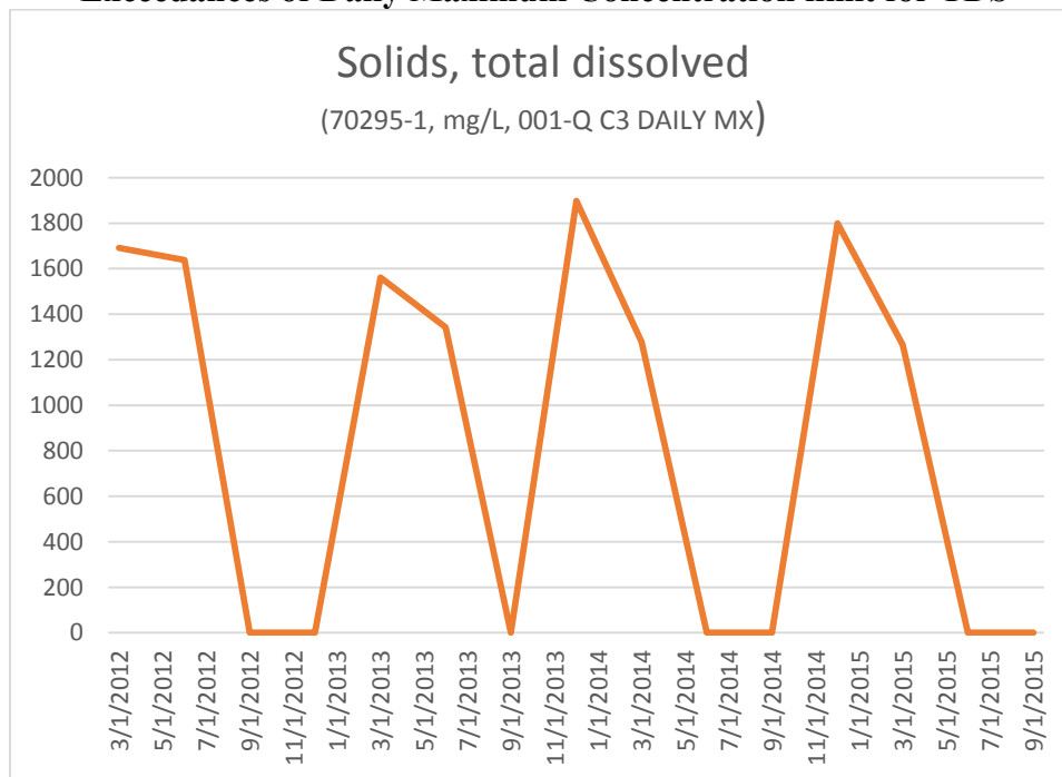
Figure 8 Exceedances of Daily Maximum Concentration limit for TDS
