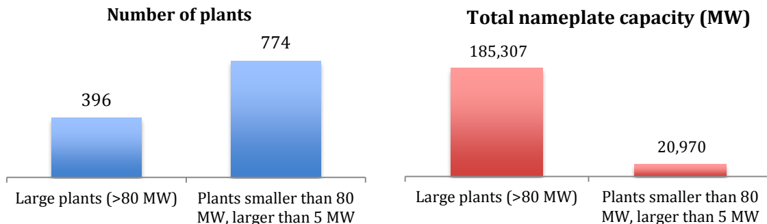
Figure 12. Distribution of generation capacity in WECC by size of plant
