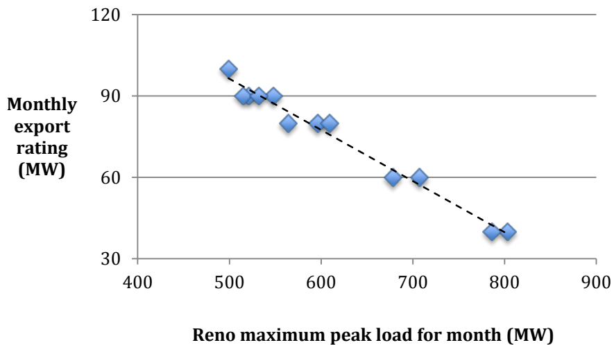
Figure 8. Path 24 export rating and Reno peak load (monthly)
