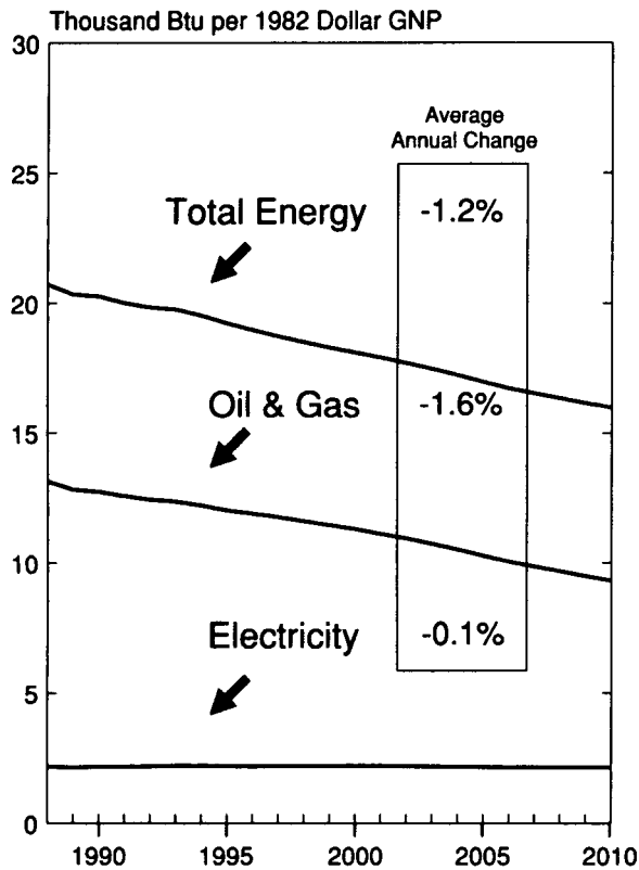
Figure 7. U.S. Energy Intensity, Base Case, 1988-2010
