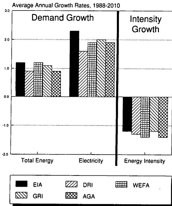
Figure 17. Annual Growth Rates for Total Energy Demand, Electricity Demand, and Total Energy Intensity, 1988-2010
