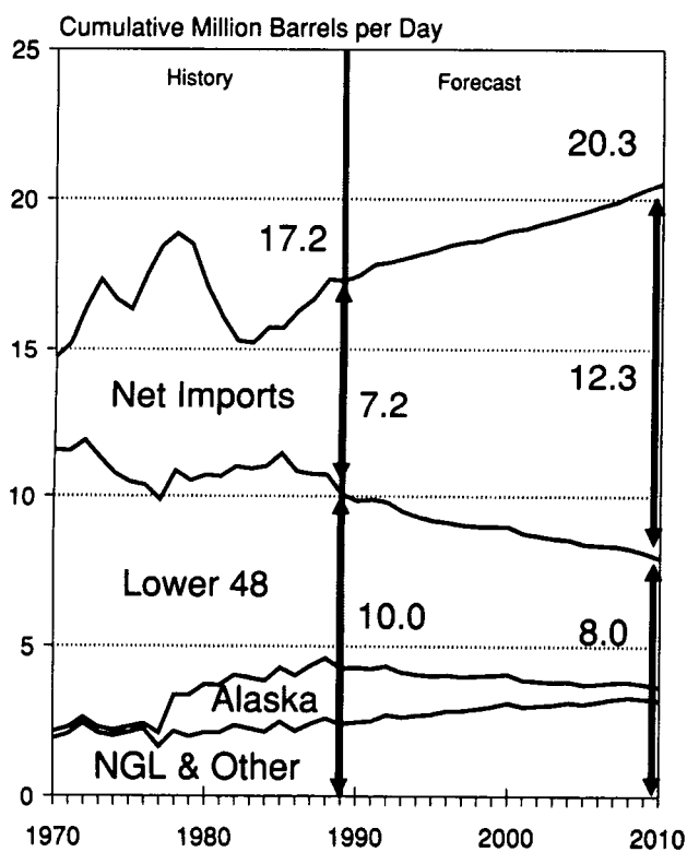
Figure 9. Petroleum Supply and Consumption, Base Case, 1970-2010
