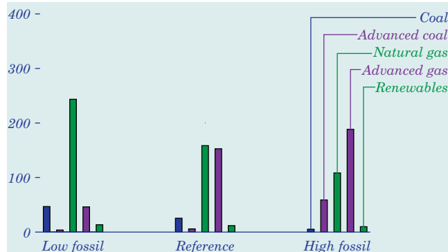
Figure 58. Projected cumulative new generating capacity by technology type in three fossil fuel technology cases, 2000-2020 (gigawatts)
