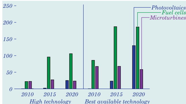
Figure 41. Buildings sector electricity generation from advanced technologies in alternative cases, 2010-2020 (percent change from reference case)
