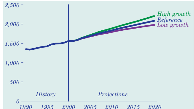
Figure 100. Projected carbon dioxide emissions in three economic growth cases, 1990-2020 (million metric tons carbon equivalent)
