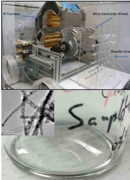
1 st Generation- Proof of concept 10KW 0.001 mg/h
