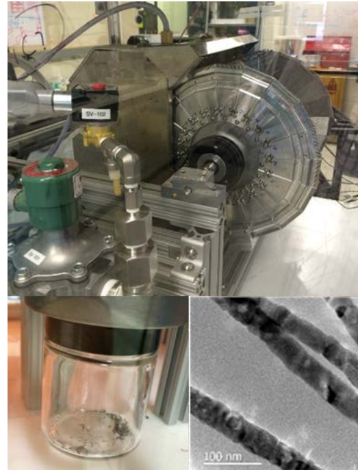
2 nd Generation- Performance improvement 6KW 0.1mg/h
