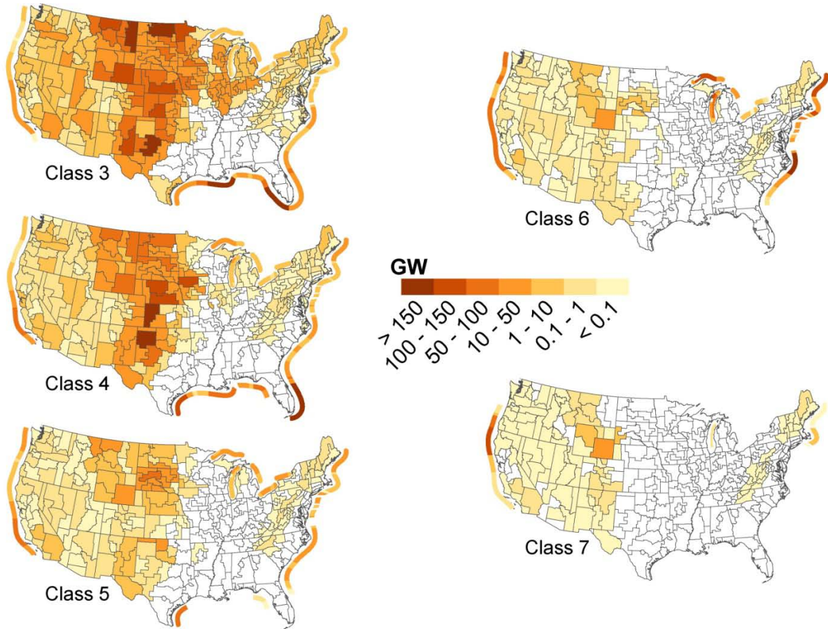
Figure 3. Available wind resource (onshore and offshore) by class
