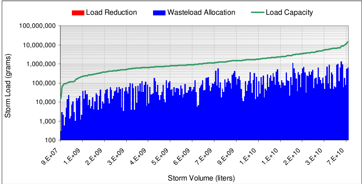
Figure 13.a. Estimated Lead Reductions to Meet Wet-Weather Grouped Storm Water Waste Load Allocations for San Gabriel River Reach 2 and Upstream Reaches and Tributaries.
