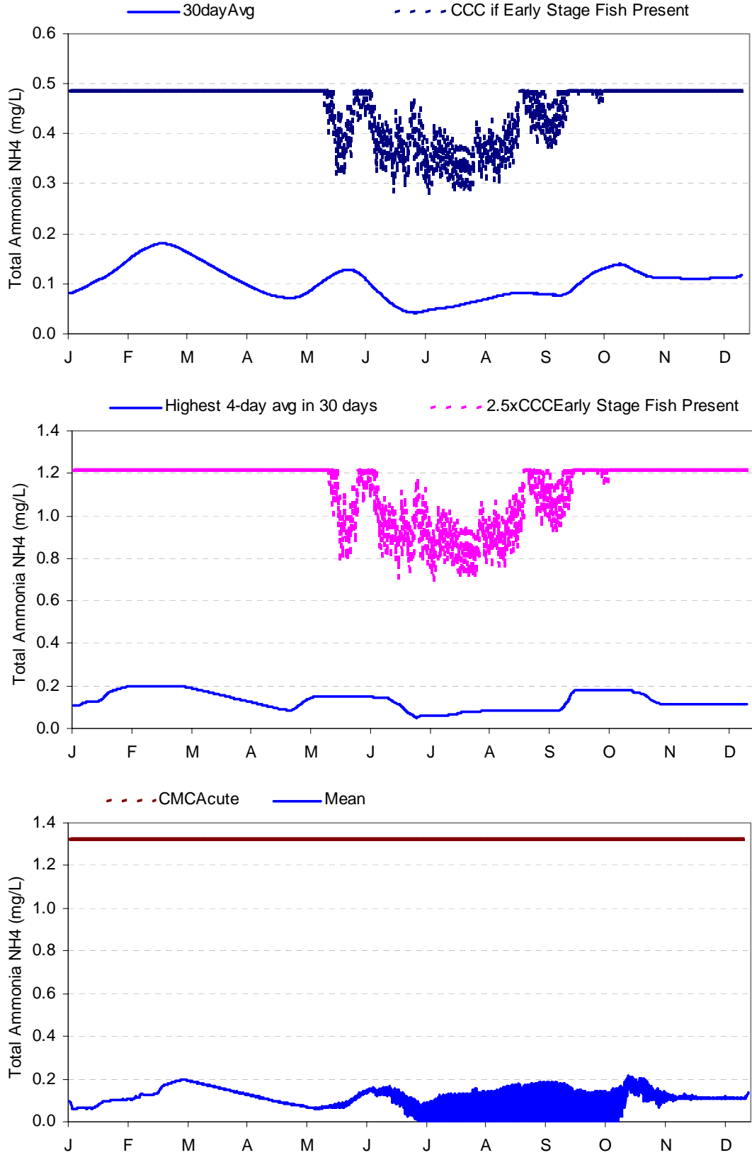
D_1999-2 Lost River at Harpold Dam (LRHD) –1999 continued
