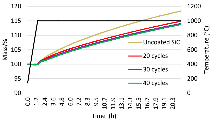
Effect of ALD Film Thickness on the Oxidation Resistance of SiC
