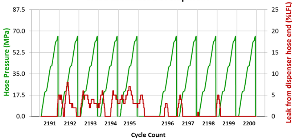
Hose Leak Rate Development
