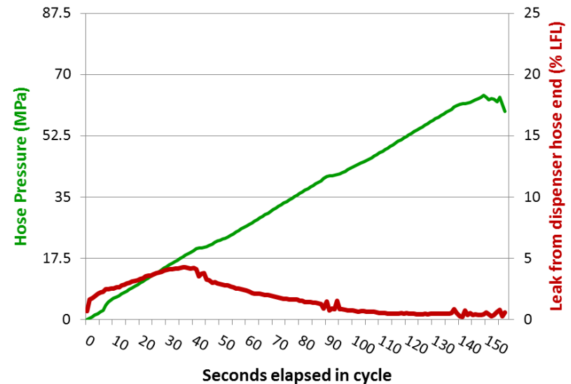
Averaged Leak Rates for Cycles 1855 to 1920
