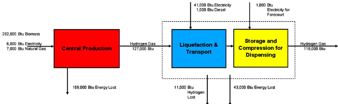
Figure 2: MSM results for hydrogen production from biomass with liquid hydrogen delivery to refueling stations
