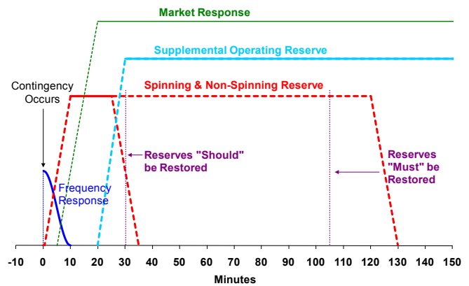
Fig. 1. Reserve deployment as defined by NERC [6]
