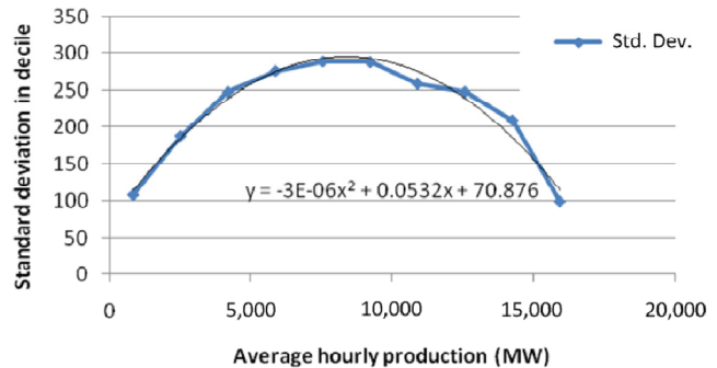
Fig. 7. 10-minute ahead wind generation forecast errors as function of production
