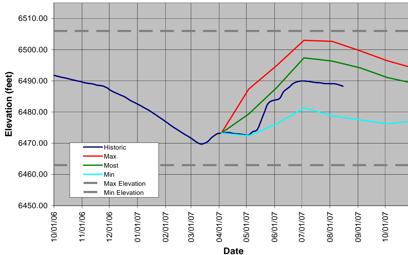
Fontenelle Reservoir 2007 Apr-Jul Elevations as of 4/5/2007
