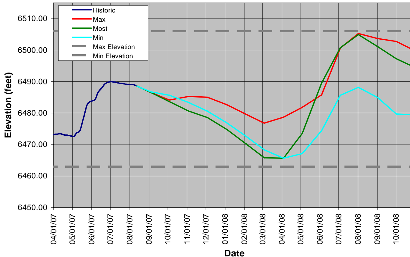
Fontenelle Reservoir 2008 Water Year Elevations Scenarios as of 8/13/2007
