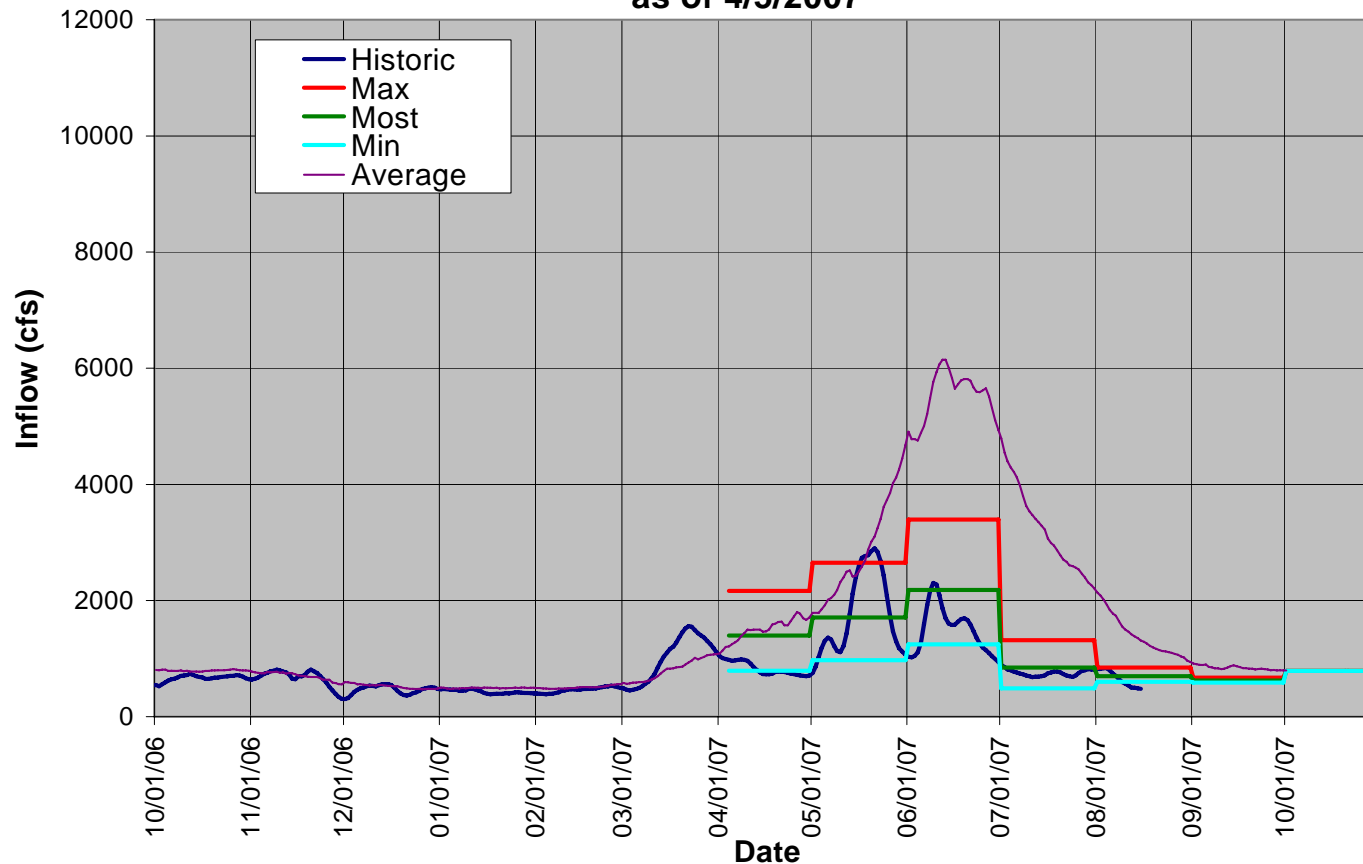
Fontenelle Reservoir 2007 Apr-Jul Inflow Scenarios as of 4/5/2007
