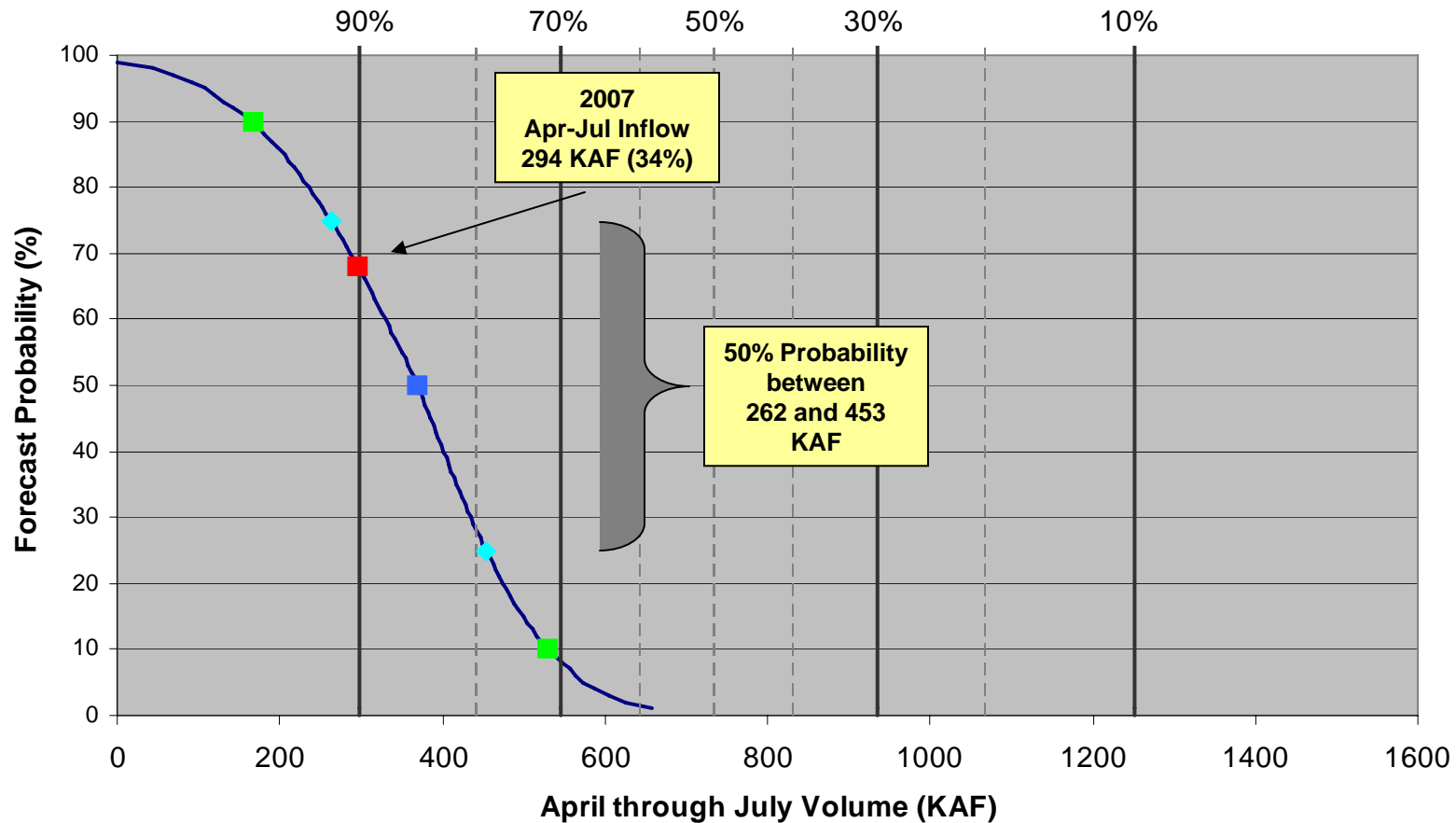
Fontenelle Reservoir 2007 Apr-Jul Forecasted Inflow (April Official Forecast) Related to Exceedance Percentages for 1976-2005 Historic Period
