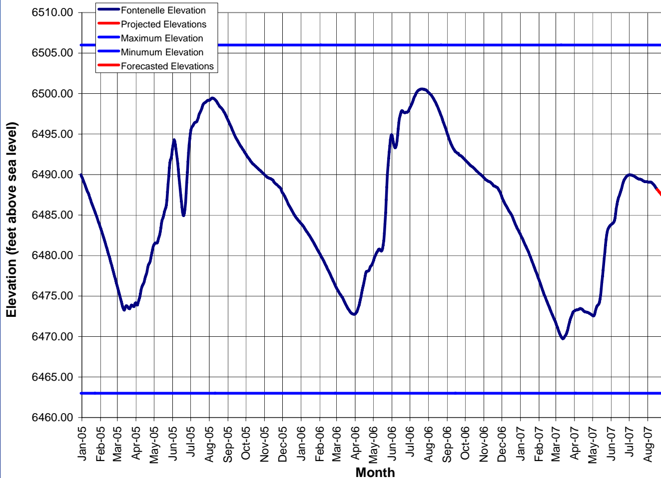
Fontenelle Operations WY2007,2008 Most Probable Operations August 2007
