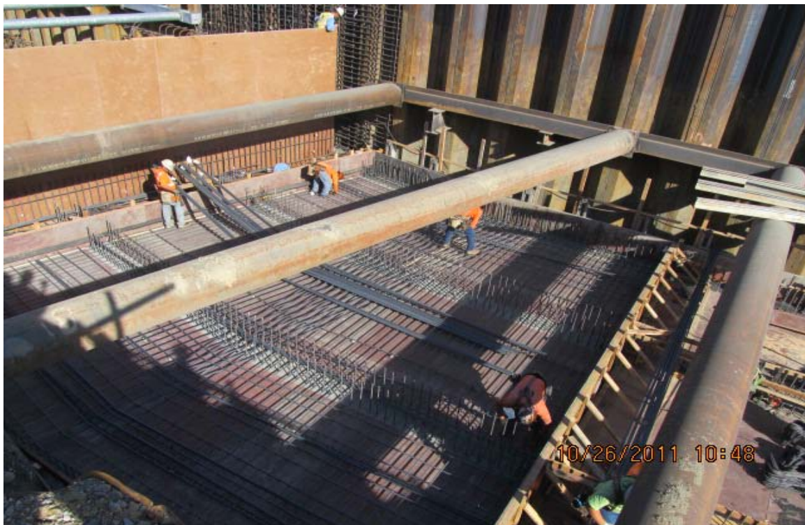
West Bay Builders subcontractor CMC Rebar installing rebar mats for Siphon Phase 3 decks.
