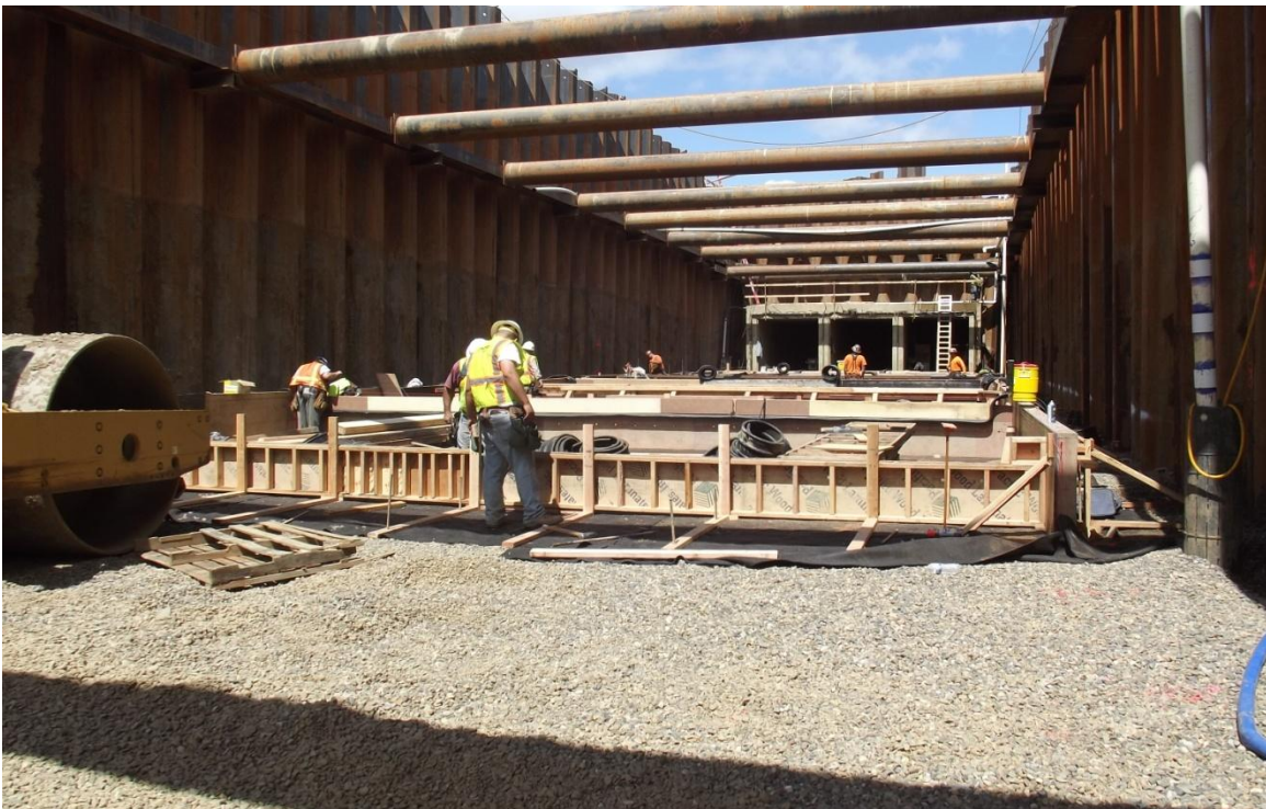
West Bay Builders carpenters setting forms for siphon concrete slab.
