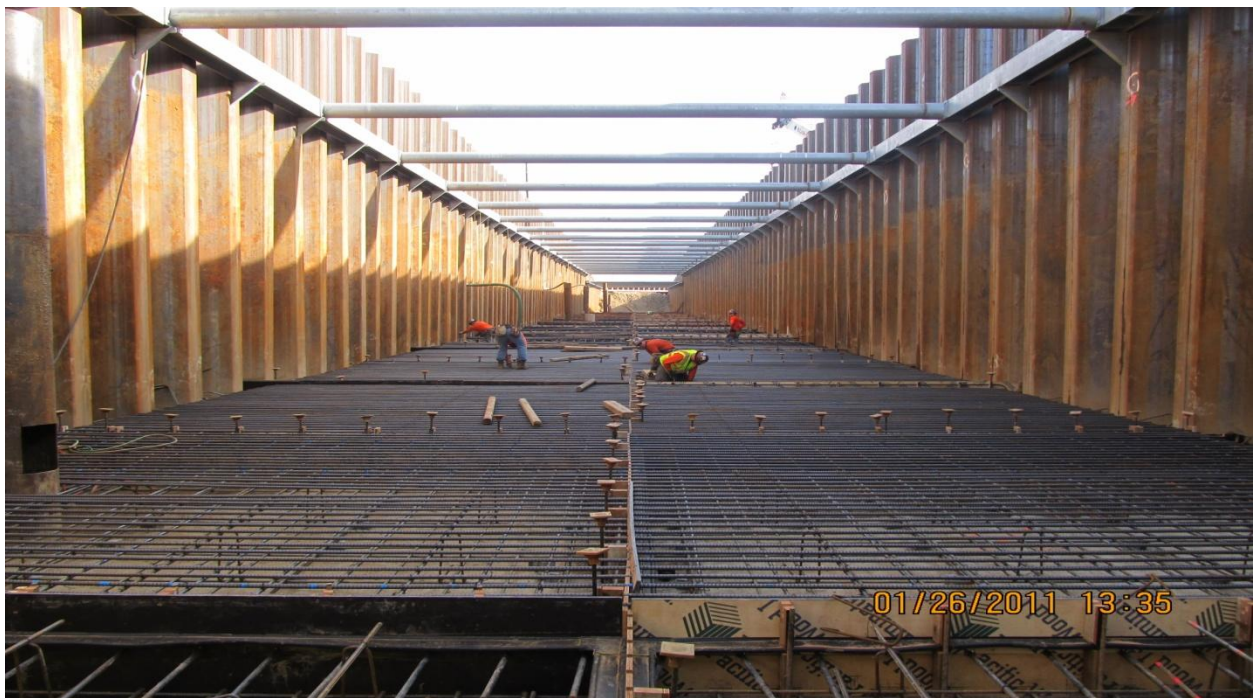
West Bay Builders Subcontractor CMC Rebar installing the top mat of the structural slab in the downstream canal.
