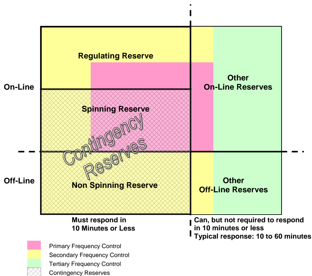
Figure 2-4. The Relationship Between Operating Reserves as Defined by NERC and Primary, Secondary, and Tertiary Frequency Control as Defined in this Study
