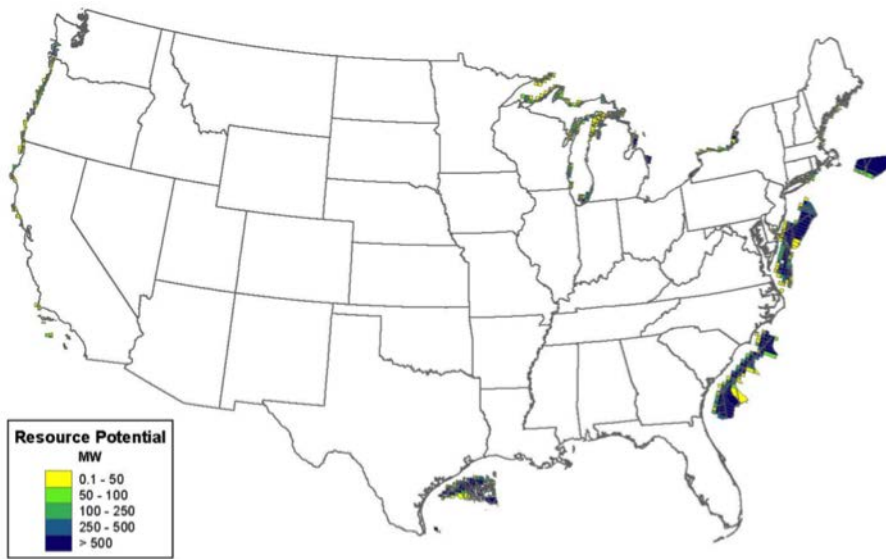
Figure H-46. Map of TRG7 (mid-depth) resource potential
