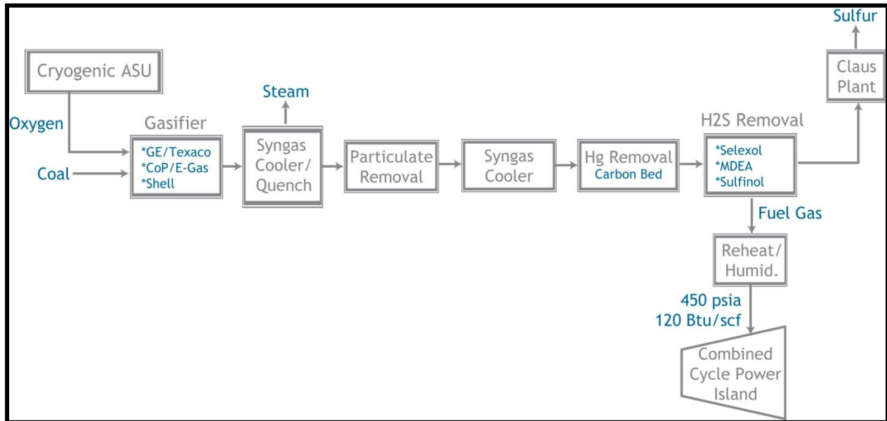
FIGURE 10-1 – IGCC DESIGN CONFIGURATION
