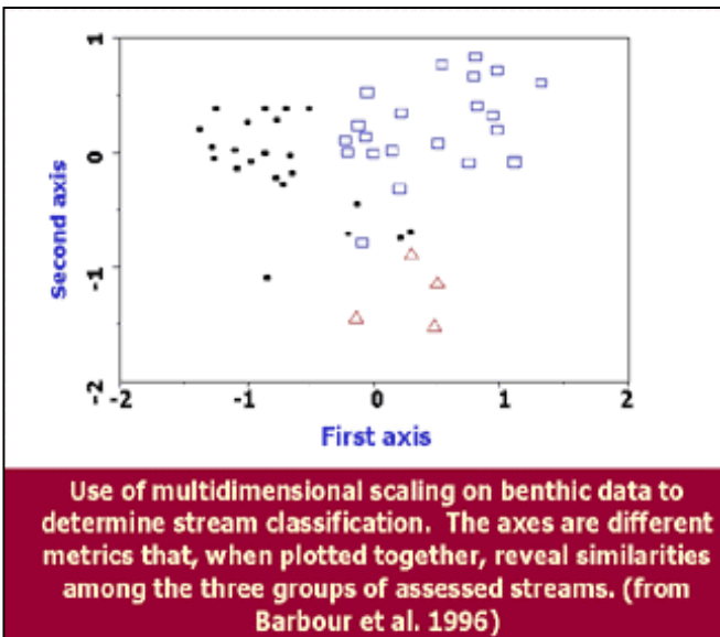
Figure 30 Bivariate scatter plots are used to compare the clustering of points using two dimensions. This technique can be used to develop regression lines or even to incorporate three factors of data.
