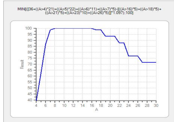
Figure 2. Age-specific % of adult females breeding used in AWB model.
