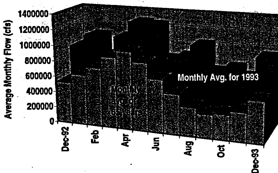
Average Monthly Flow of Mississippi River at Vicksburg for December 1992-December 1993 vs. Average of Monthly Flows for 65 year period from 1931 to 1995
