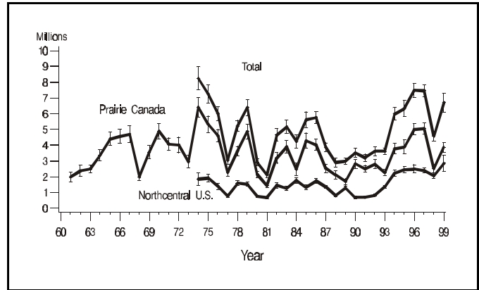
Fig. 1. Number of ponds in May and 95% confidence intervals for Prairie Canada and the northcentral U.S.
