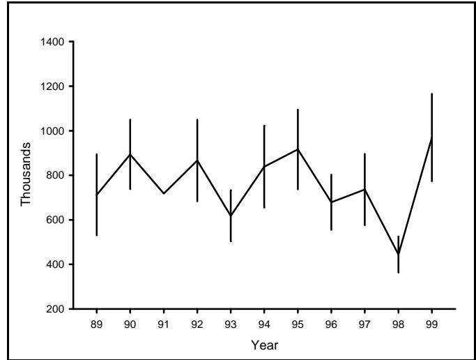
Fig. 8. Estimated size (and 95% confidence intervals) of the Mississippi Valley Population of Canada geese during spring.
