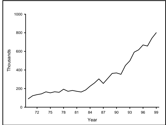
Fig. 18. Size of the Greater Snow goose population estimated from spring surveys.
