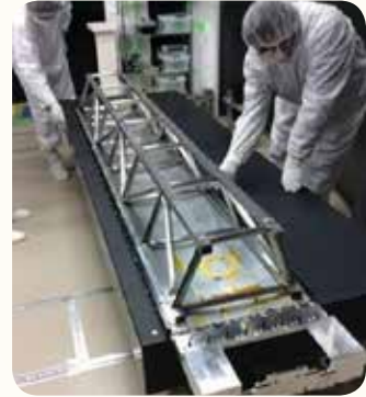
Constructed iTOP module augmented by external "strong back" to stiffen it until installation. Sixteen such modules will form a cylinder within the Belle II detector. The last module is slated for installation in spring 2016.
