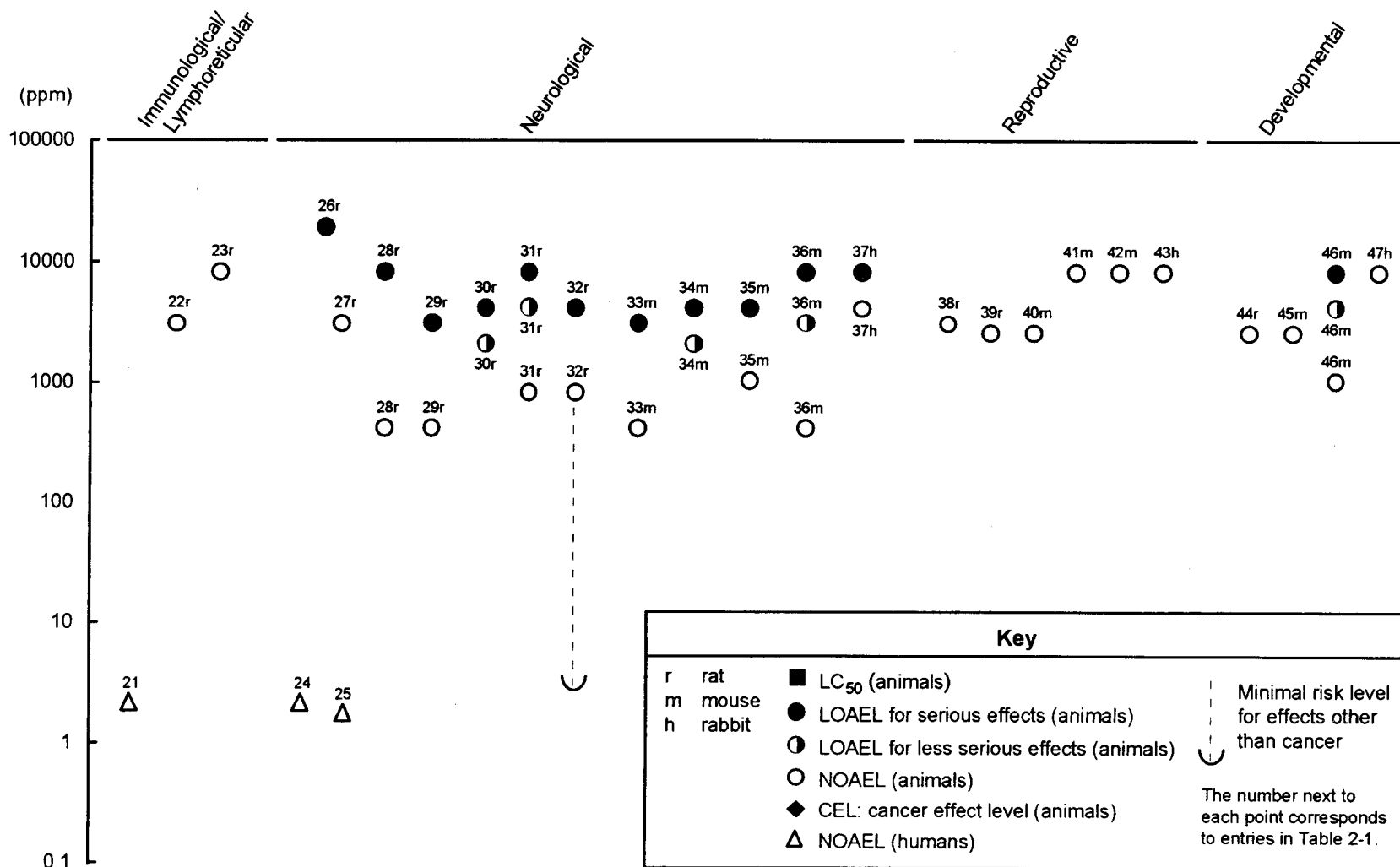
Figure 2-1. Levels of Significant Exposure to Methyl tert -Butyl Ether (MTBE) - Inhalation (cont.) Acute ( \leq 14 days)
