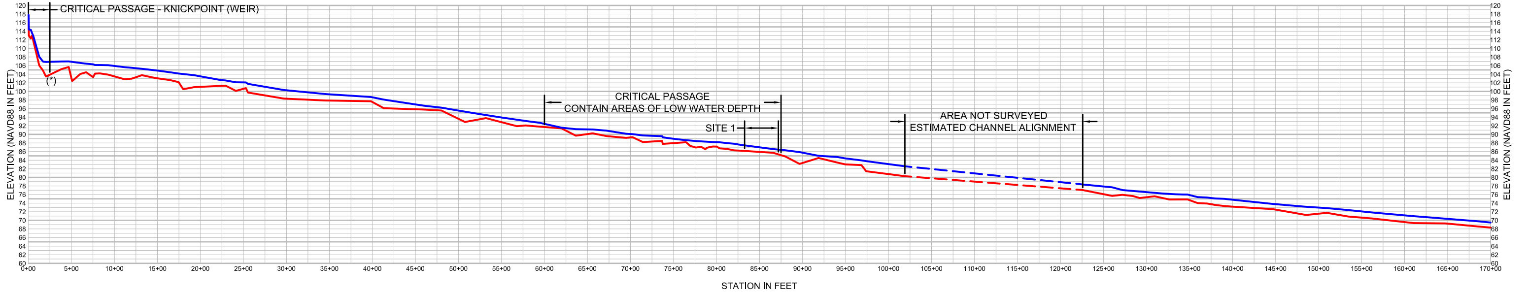
THALWEG PROFILE FROM STA:0+00 TO STA:170+00
