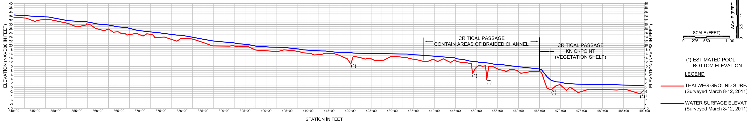
THALWEG PROFILE FROM STA:340+00 TO STA:490+00
