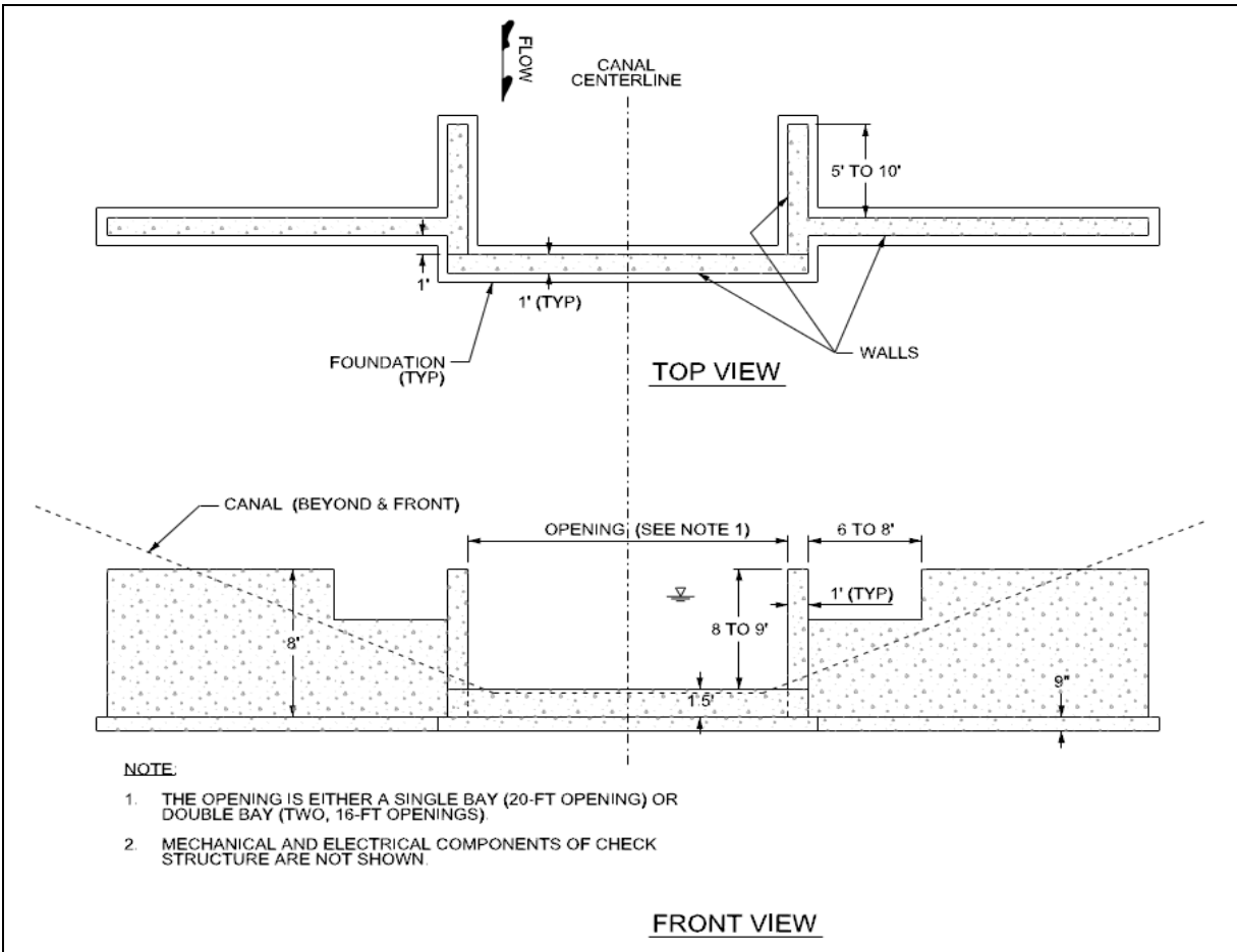
Figure 2-17. Typical Canal Check Structure
