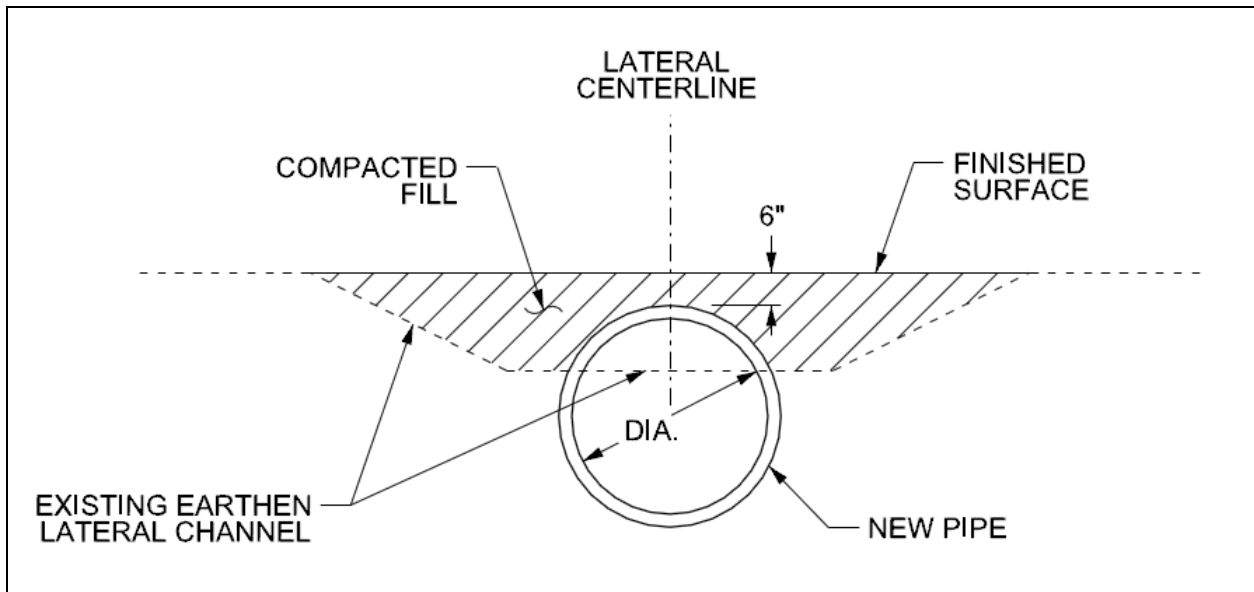
Figure 2-18. Typical Pipe Replacement Section
