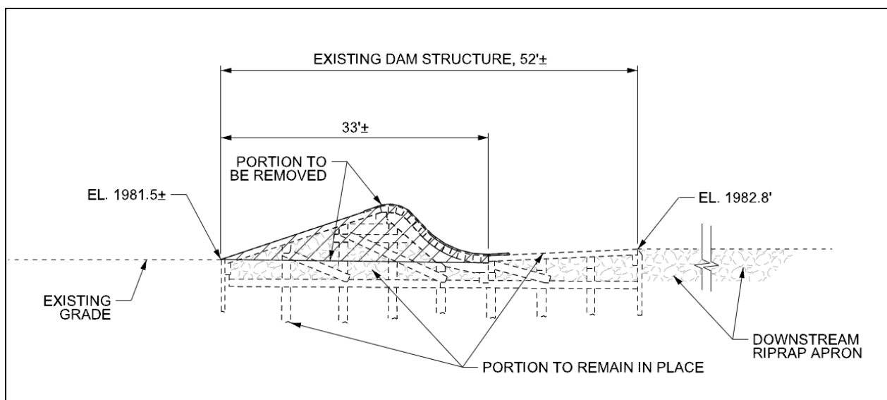
Figure 2-22. Typical Dam Removal Section
