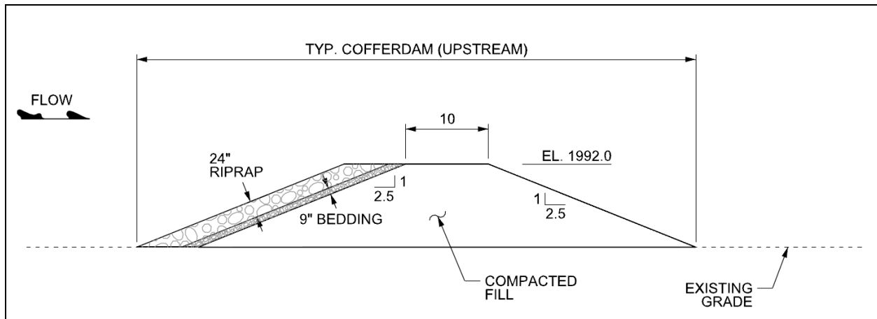
Figure 2-23. Typical Cofferdam Section
