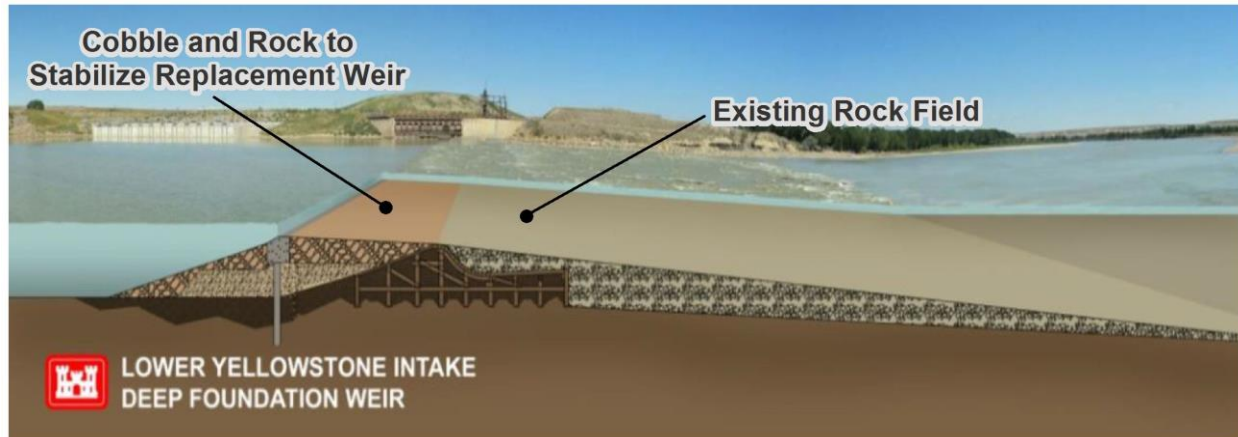
Figure 2-5. Rendering of the Replacement Weir
