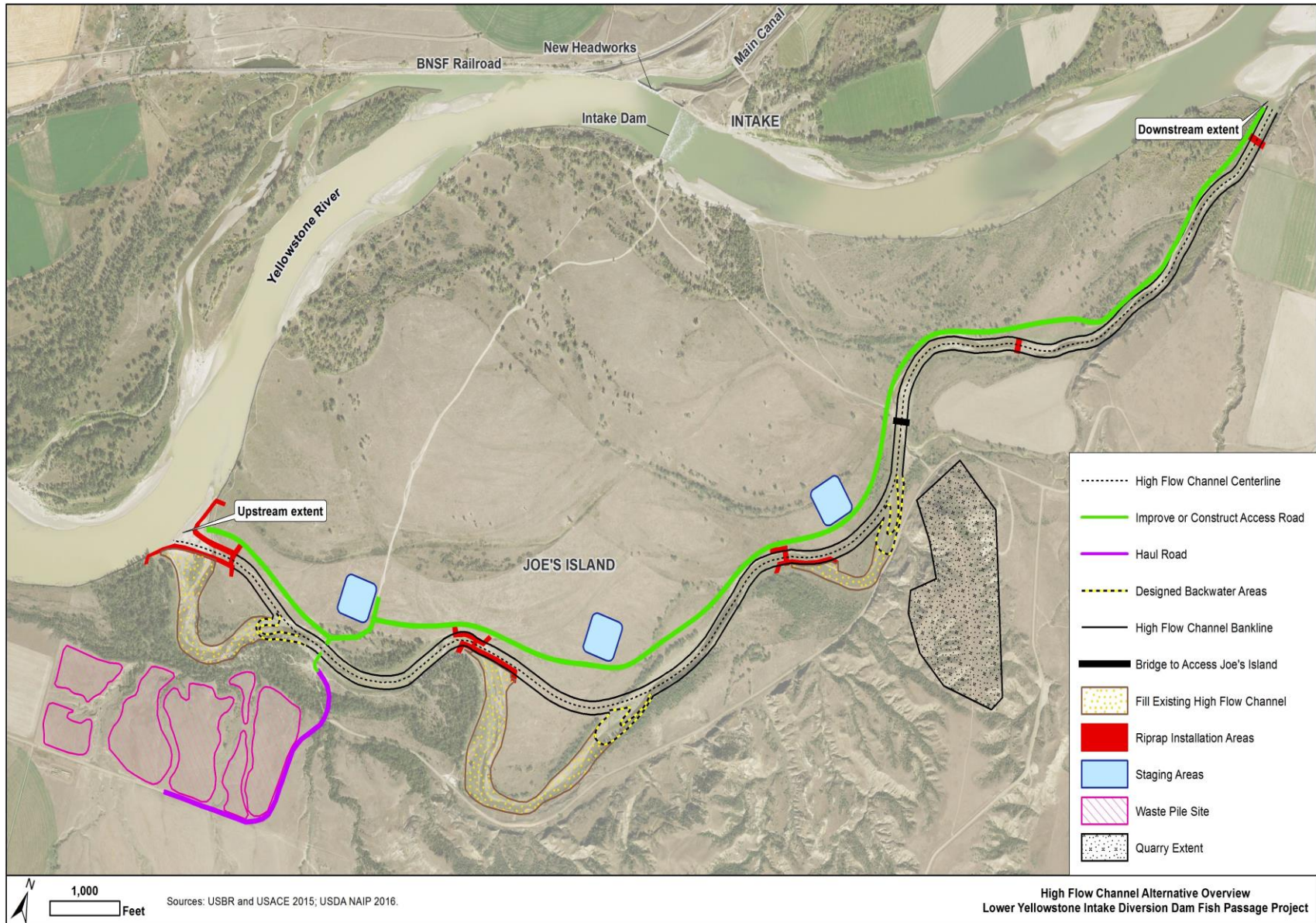
Figure 2-6. Modified Side Channel Alternative
