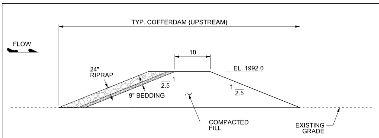
Figure 2-14 Typical Cofferd Dam Section
