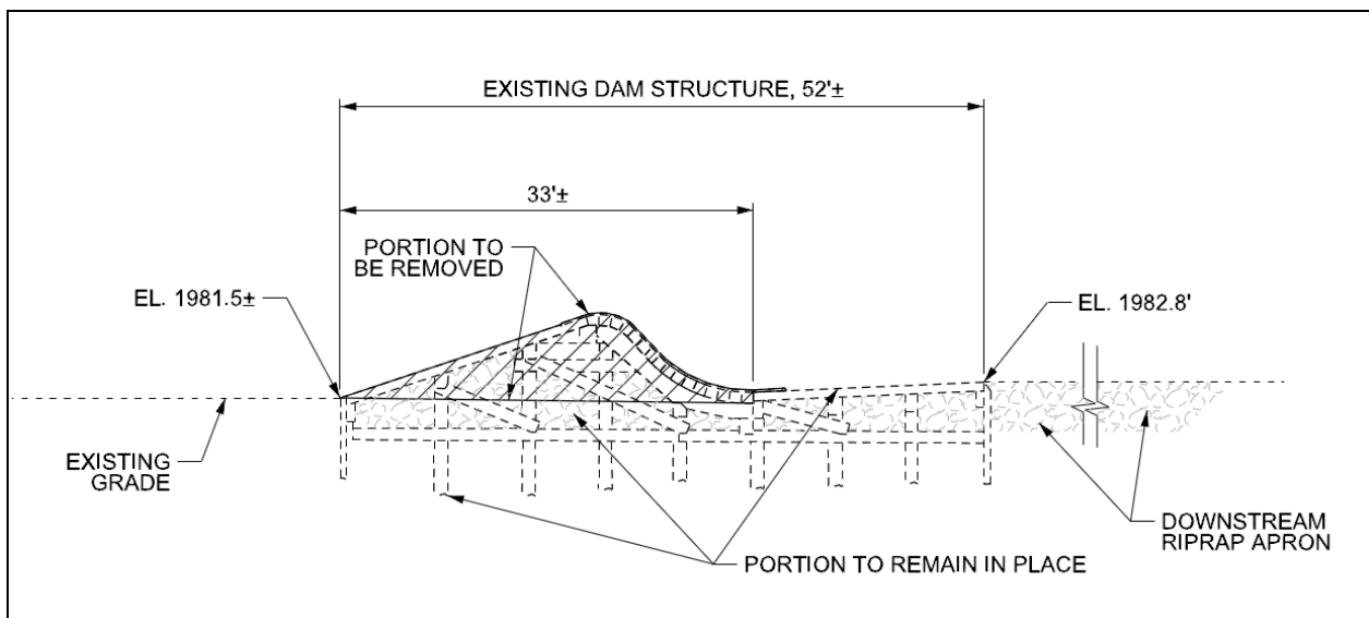
Figure 2-13 Typical Dam Removal Section
