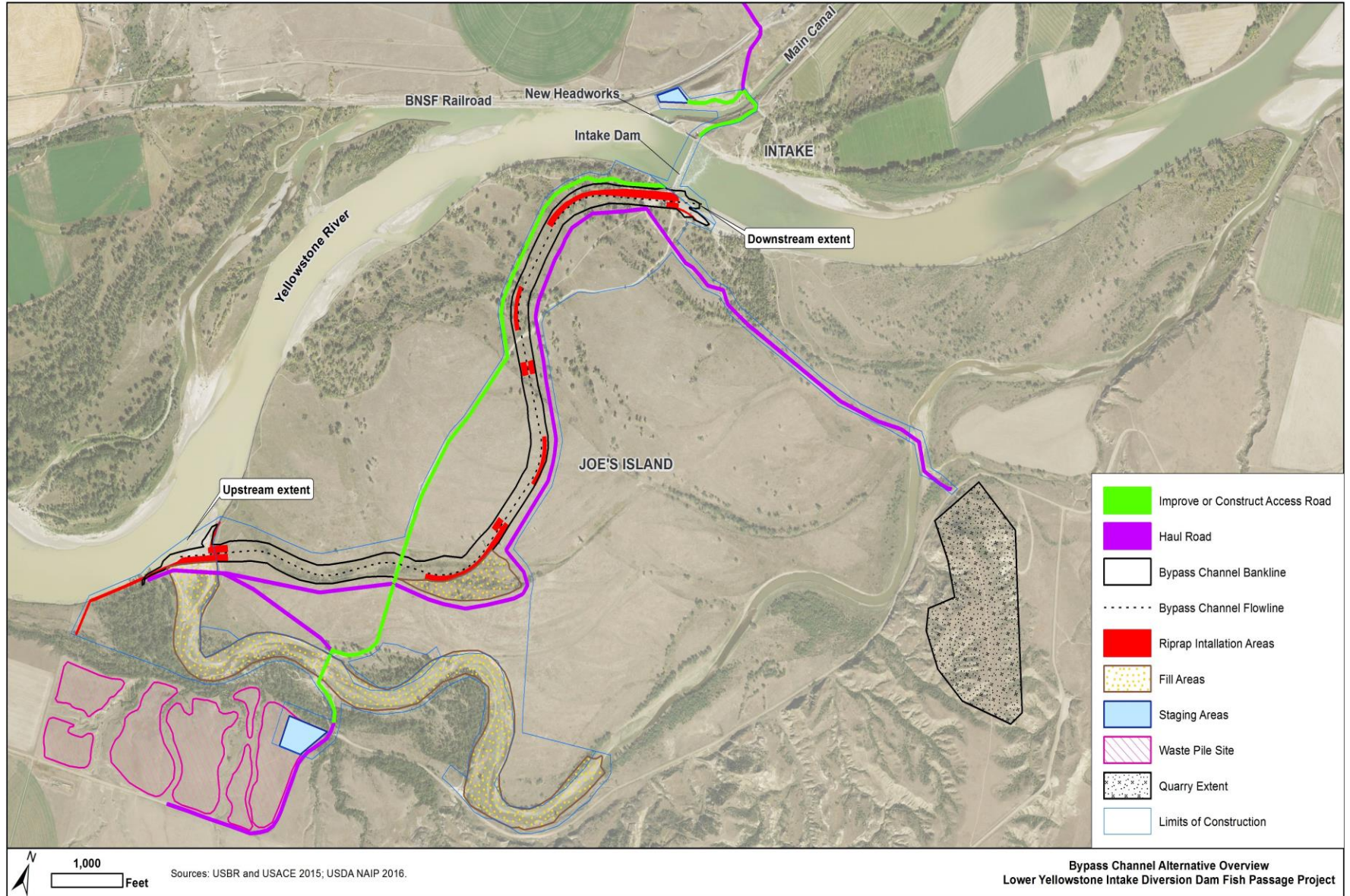
Figure 2-4. Bypass Channel Alternative Overview
