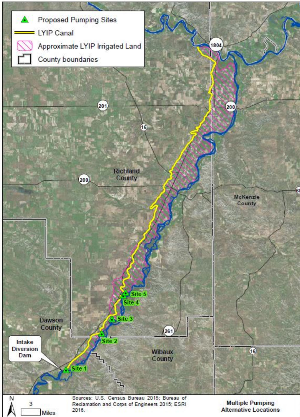
Figure 2-10. Multiple Pumping Station Locations
