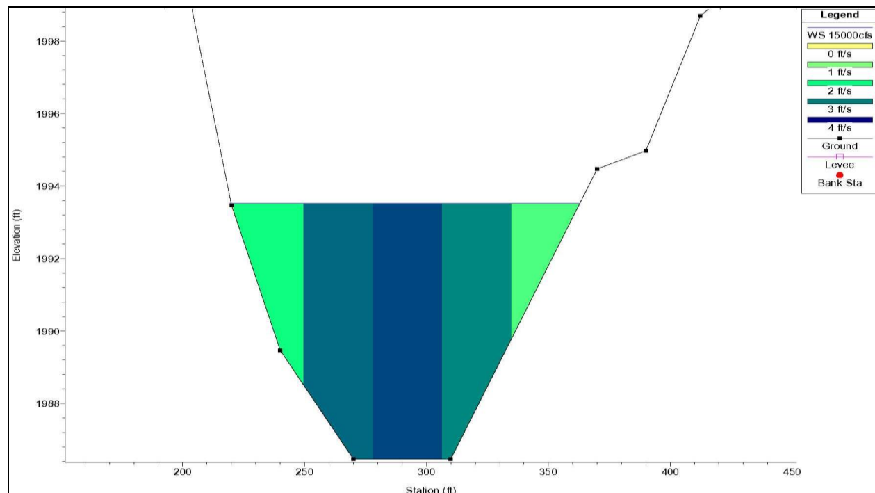
Figure 4-3. Typical Modeled Mean Column Velocity for the Bypass Channel Alternative
