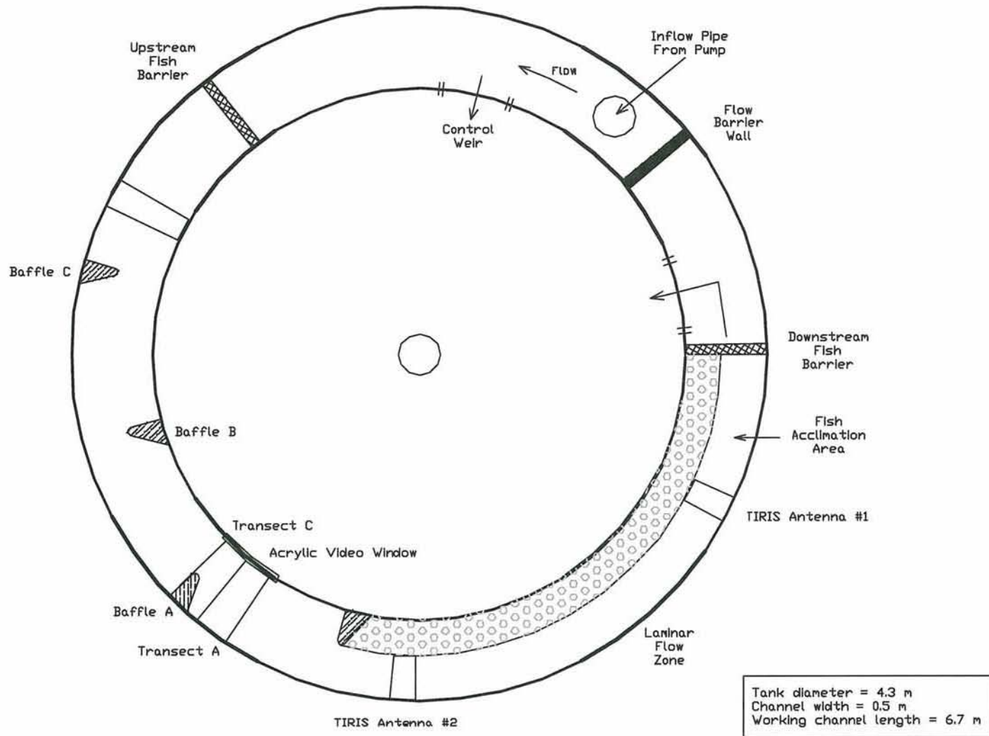
Figure 1. Experimental flume with different flow conditions (up- to downstream): structure/turbulent flow within the baffle area, then laminar flow with decreasing velocity to the acclimation area.
