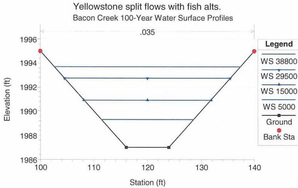
Figure 3 Typical Section from Riprap Fish Ladder Model
