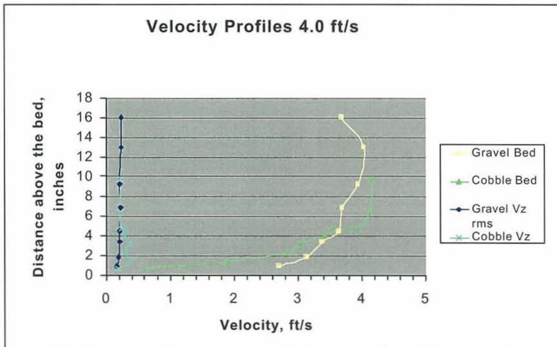
Figure 15 - Vertical velocity profiles measured over gravel and cobble beds for flume tests with an average flow velocity target of 4.0 ft/s.
