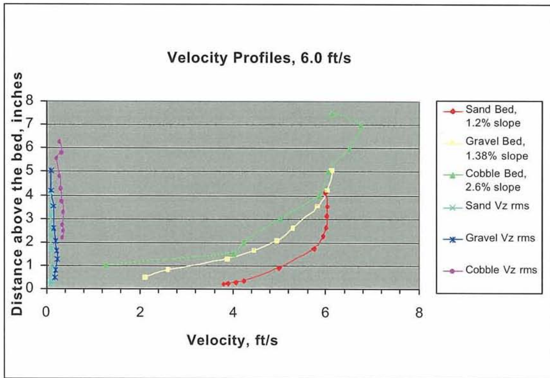
Figure 16 - Vertical velocity profiles measured over coarse sand, gravel and cobble beds for flume tests with a target average flow velocity of 6.0 ft/s.
