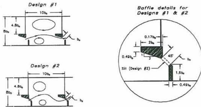
View of standard vertical slot baffle fishway looking downstream.
