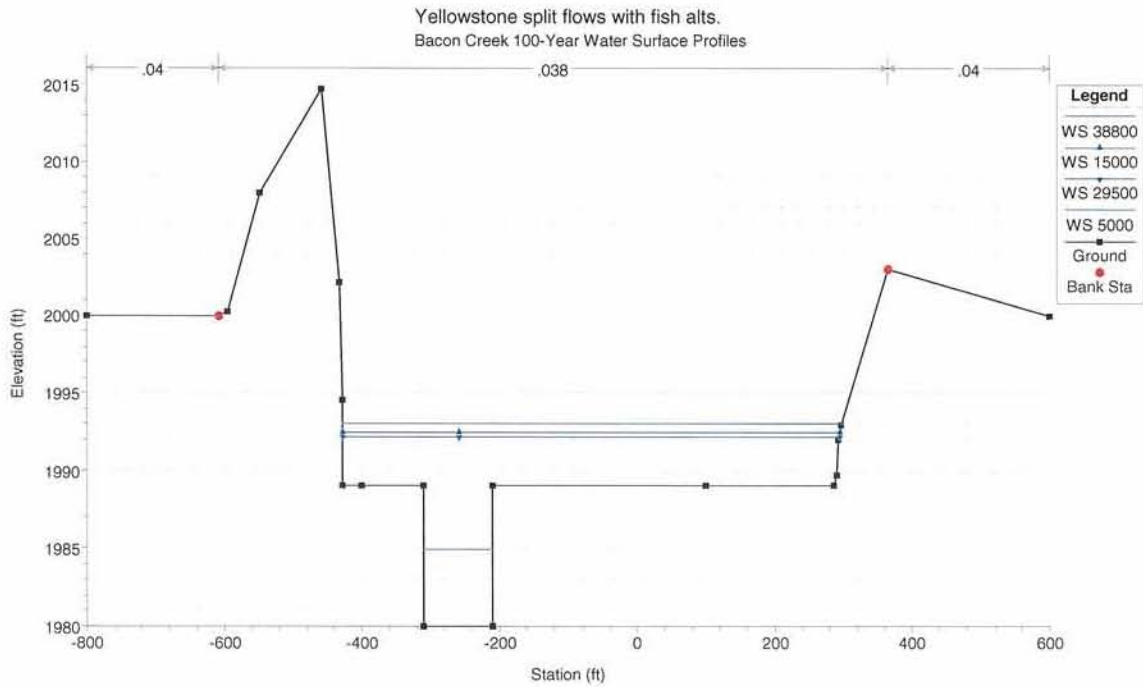
Figure 14 Cross Section at Embankment for Collapsible Gates with Five Gate Fully Lowered
