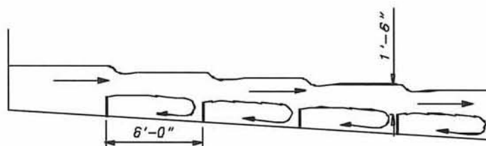
Figure 20 - Elevation view of flow over weir baffles in the test flume.
