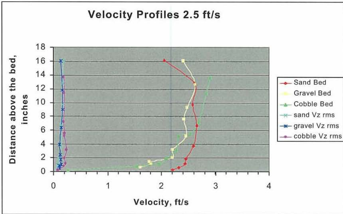
Figure 12 - Vertical velocity profiles measured over coarse sand, gravel and cobble beds for flume tests with an average flow velocity target of 2.5 ft/s.
