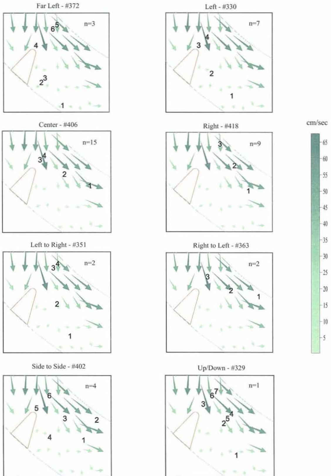
Figure 10. Eight movement routes through the baffle slot as shown by a typical fish (numbered). Total number of fish trips with each route (n) shown inside figure.
