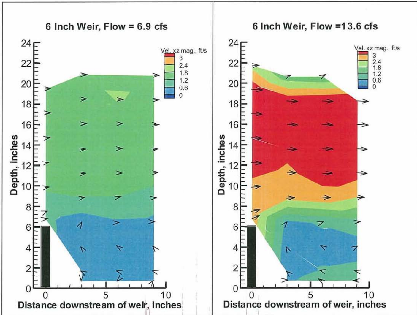
Figure 22 - Elevation view of measured velocity vector field downstream of 6 inch high weir baffles.
