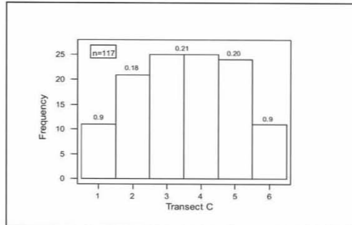
Figure 11. Movement of fish passing through the "video zone" as shown by the frequency of occurrence of fish passing across transects A-B (downstream of baffle slot) and transect C (baffle slot). Probability of occurrence is above each bar; n = total number of observations of all fish and all trips. Position 1 is on outside wall, position 6 and 11 are on inside wall.
