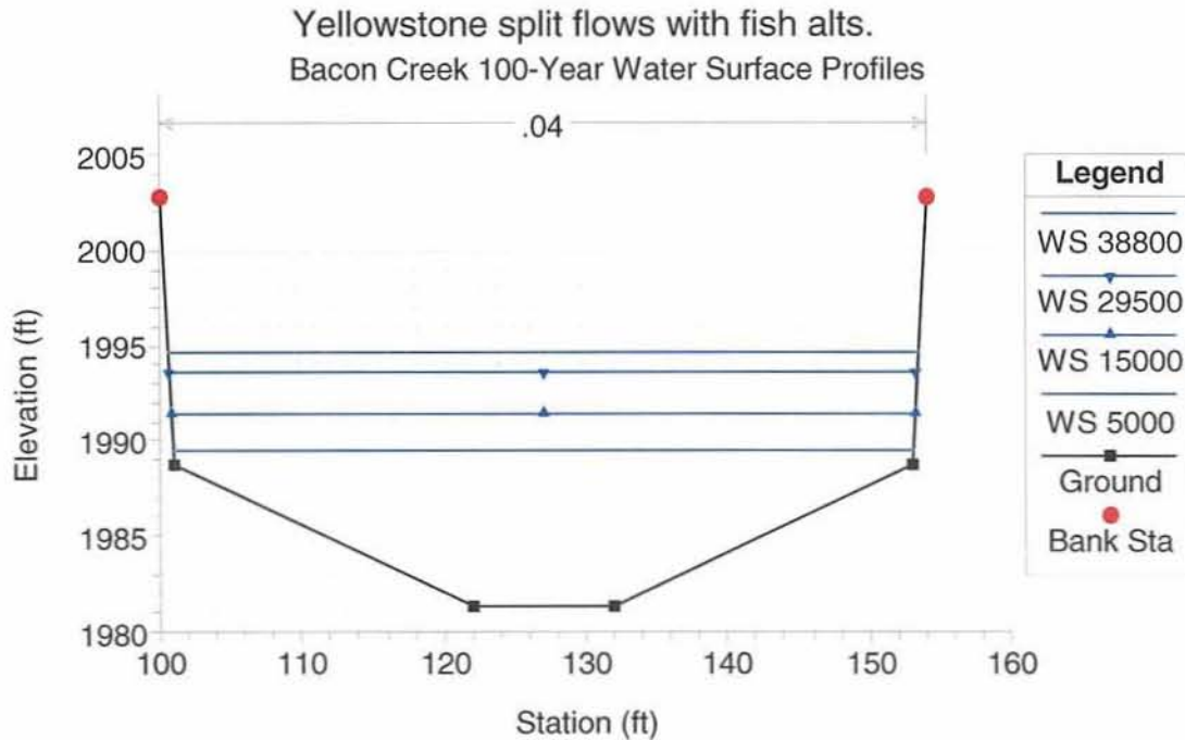
Figure 5 Typical Section from Riprap Fish Ladder Model
