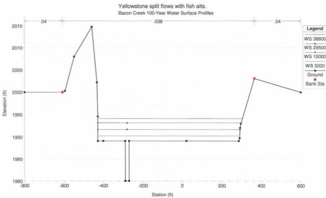
Figure 12 Cross Section at Embankment for Collapsible Gates with One Gate Fully Lowered
