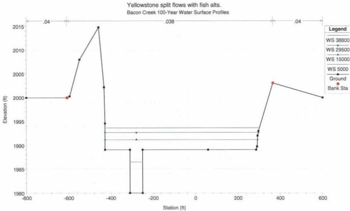
Figure 13 Cross Section at Embankment for Collapsible Gates with Three Gate Fully Lowered
