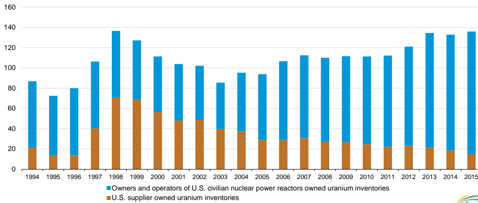
Figure S5. Total commercial uranium inventories of U.S. suppliers and owners and operators of U.S. civilian nuclear power reactors, 1994-2015 million pounds U 3 O 8 equivalent
