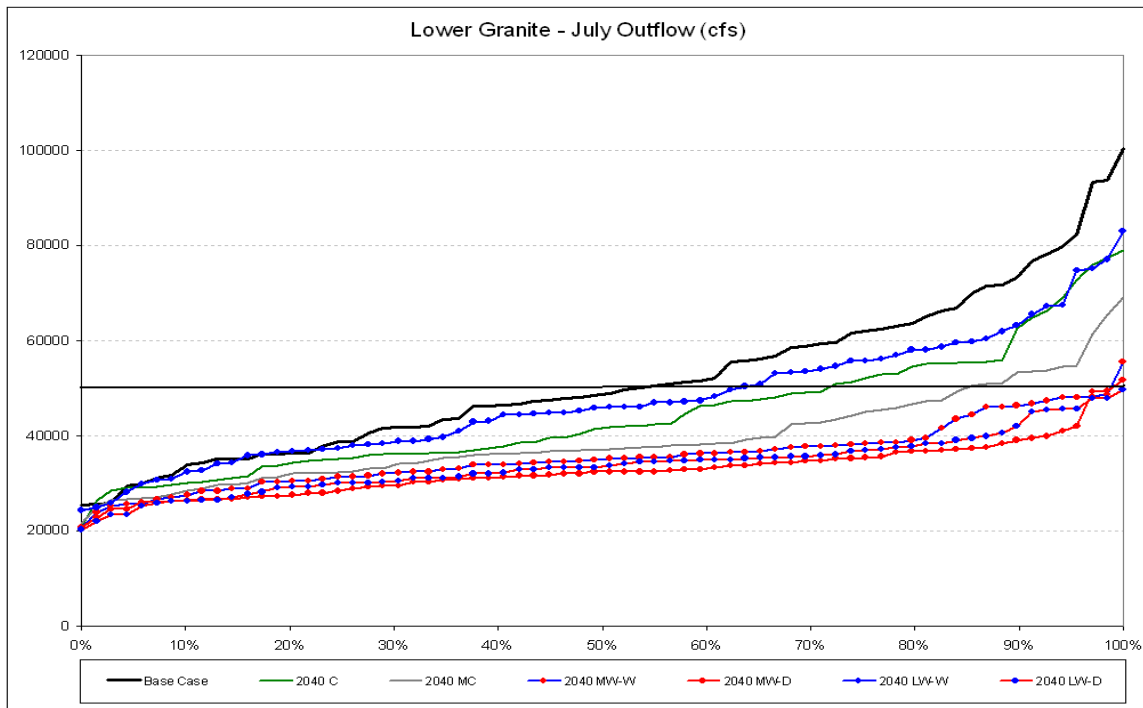
Figure 140. Comparison of 2040 Hybrid-Delta scenarios - July Lower Granite outflow distributions
