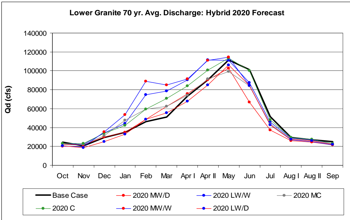
Figure 121. Lower Granite Discharge: 2020s Hybrid-Delta.
