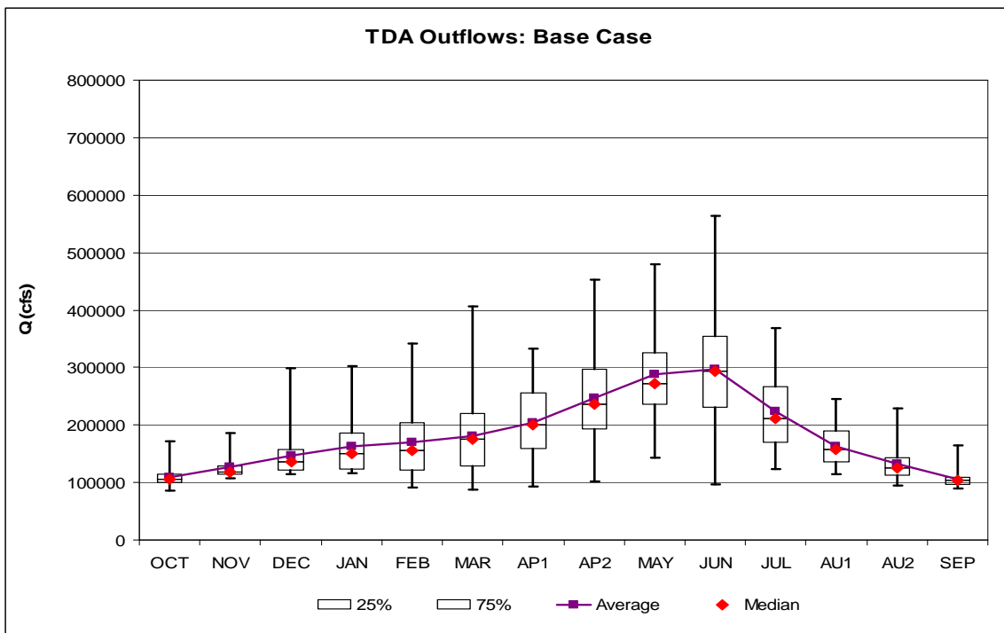
Figure 129. The Dalles Outflows for Base Case.
