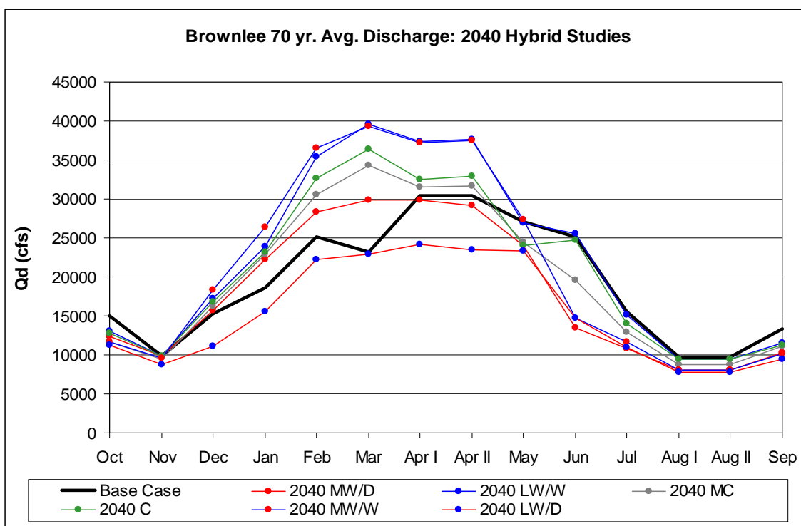
Figure 118. Brownlee monthly average discharge for each 2040 Hybrid-Delta climate change scenario.
