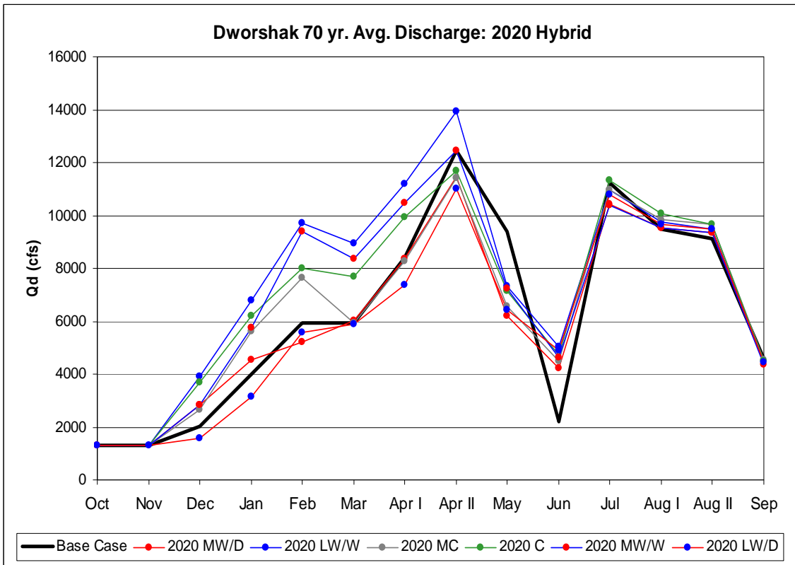
Figure 108. Dworshak seventy-year averaged Discharge: 2020s Hybrid-Delta.
