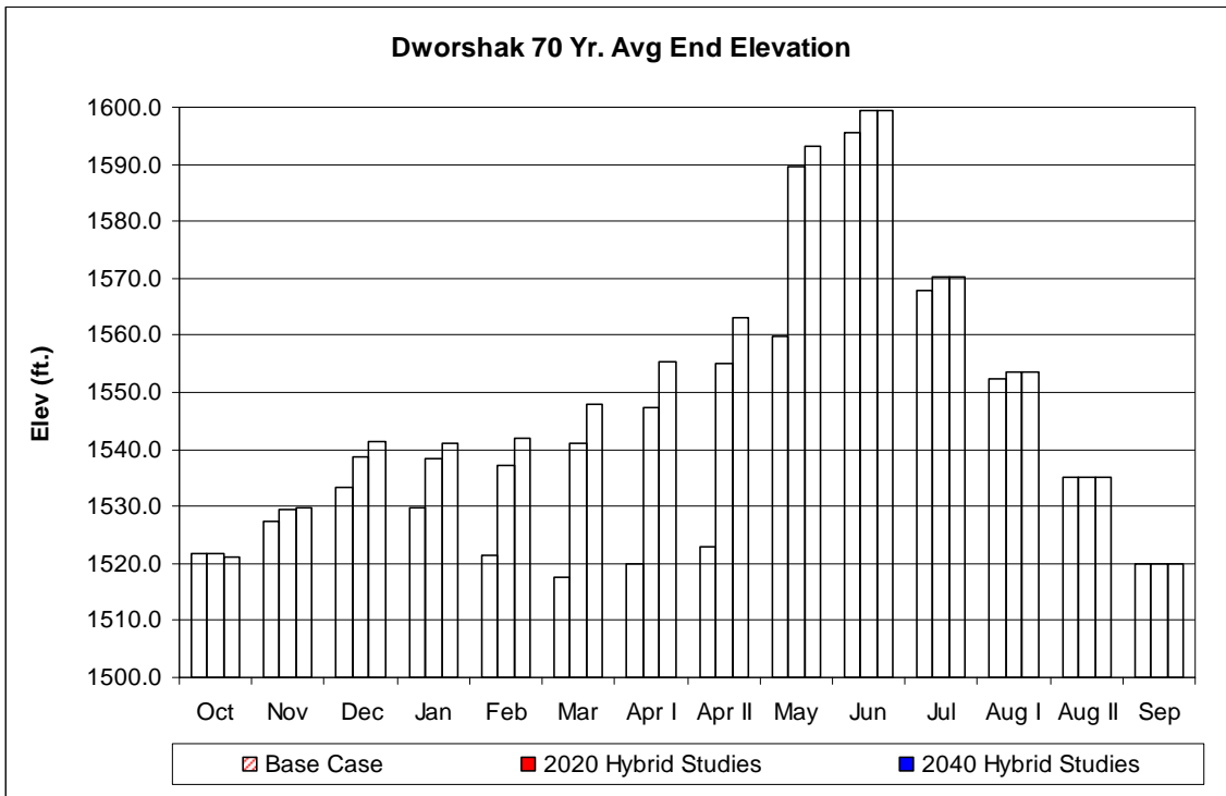
Figure 106. Dworshak Average End Elevation for Base Case and Climate Change Scenarios.
