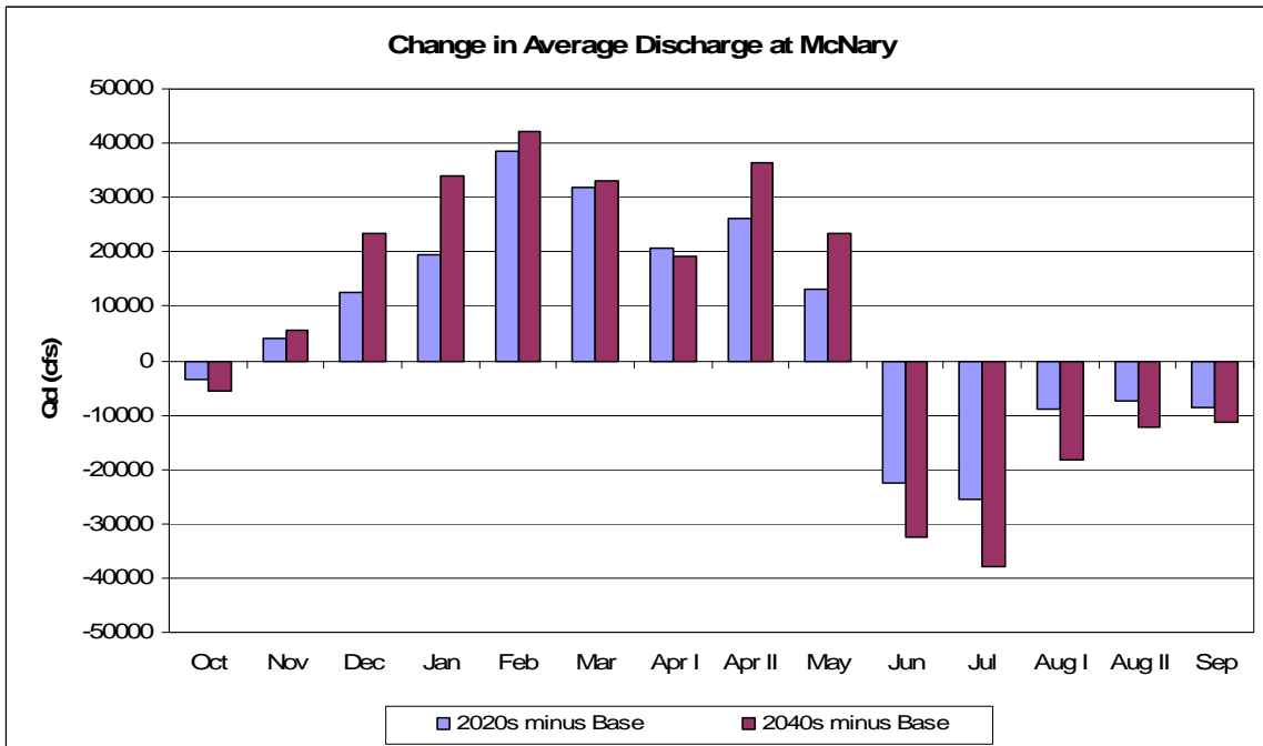
Figure 125. McNary Avg. Mo. Discharge Delta for Base Case and Hybrid-Delta Climate Change Scenarios.
