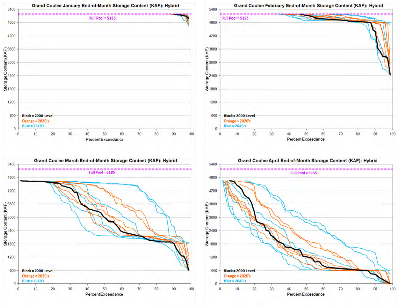
Figure 35. GCL Flood Control Storage Exceedance – Hybrid-Delta.
