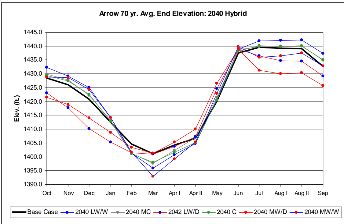
Figure 78. Arrow End Elevation: 2040s Hybrid-Delta.
