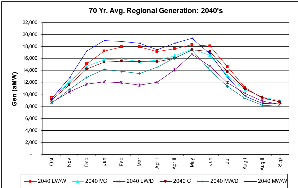
Figure 166. Regional System Generation for Hybrid-Delta 2040s Scenarios.
