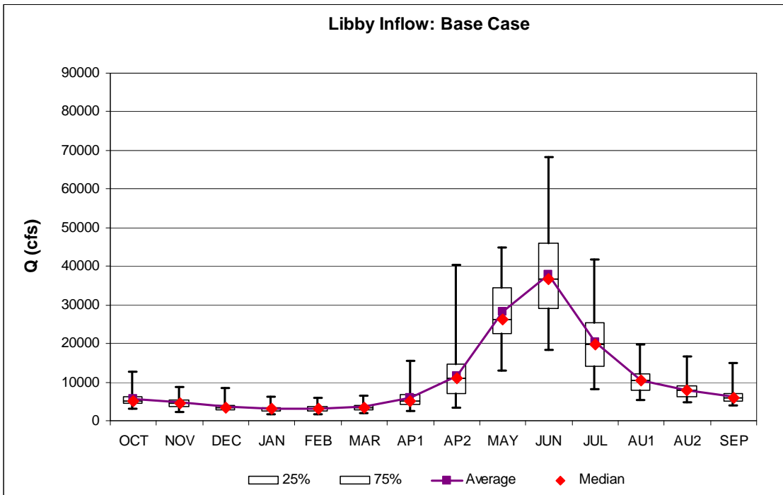
Figure 88. Libby Base Case 70 year natural inflow distribution.
