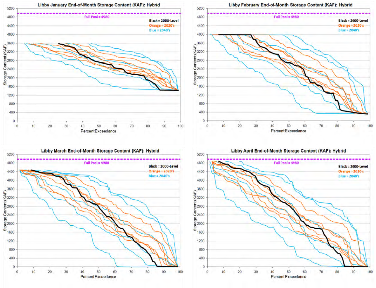
Figure 49. Libby Flood Control Storage Exceedance – Hybrid-Delta.
