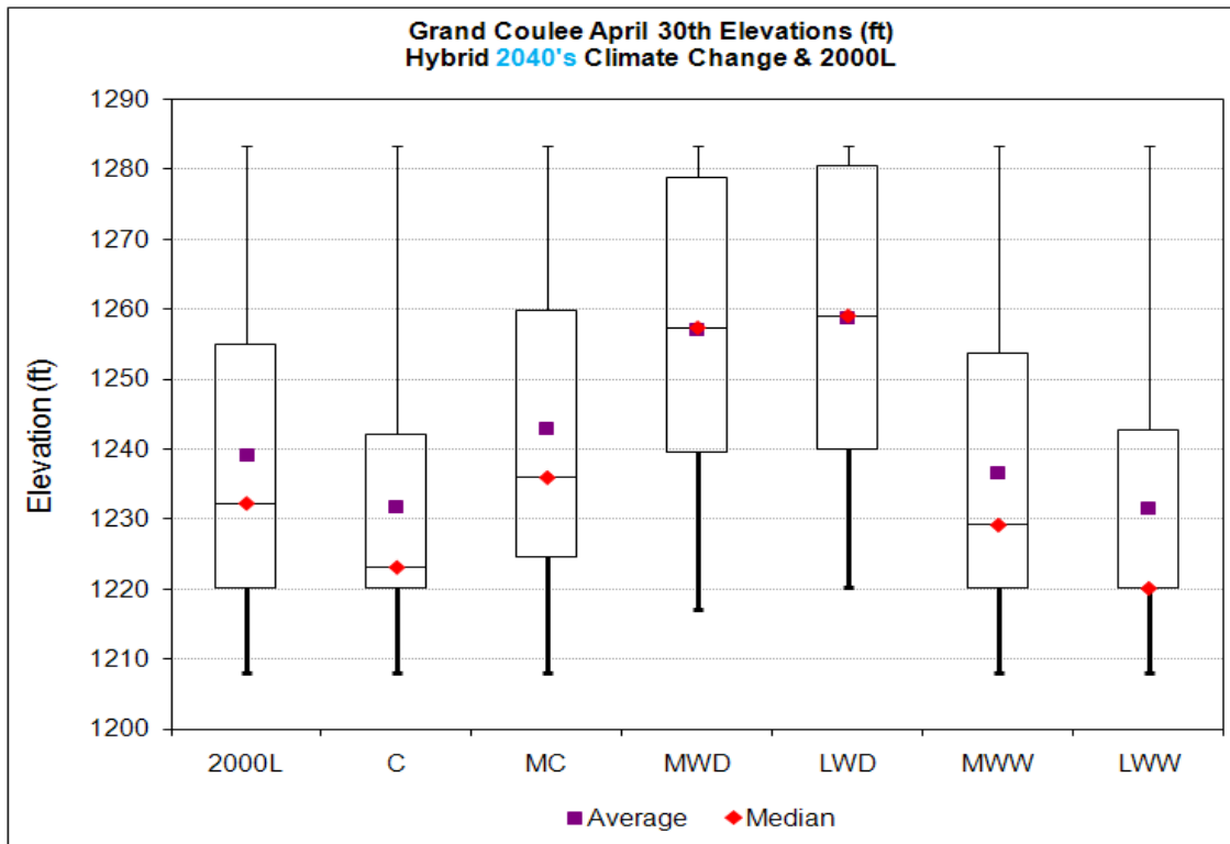
Figure 37. Grand Coulee April 30th Elevations, 2000 Level & Climate Change Scenarios–HD 2040s.
