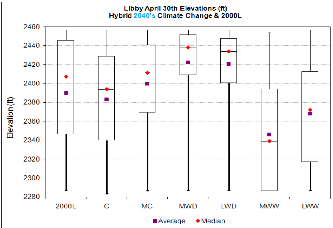
Figure 51. Libby April 30th Elevations, 2000 Level & Climate Change Scenarios – Hybrid-Delta 2040s.
