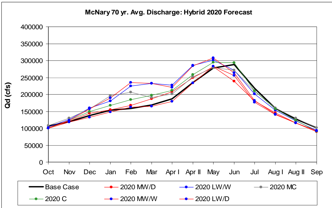
Figure 126. McNary Discharge: Hybrid-Delta 2020s
