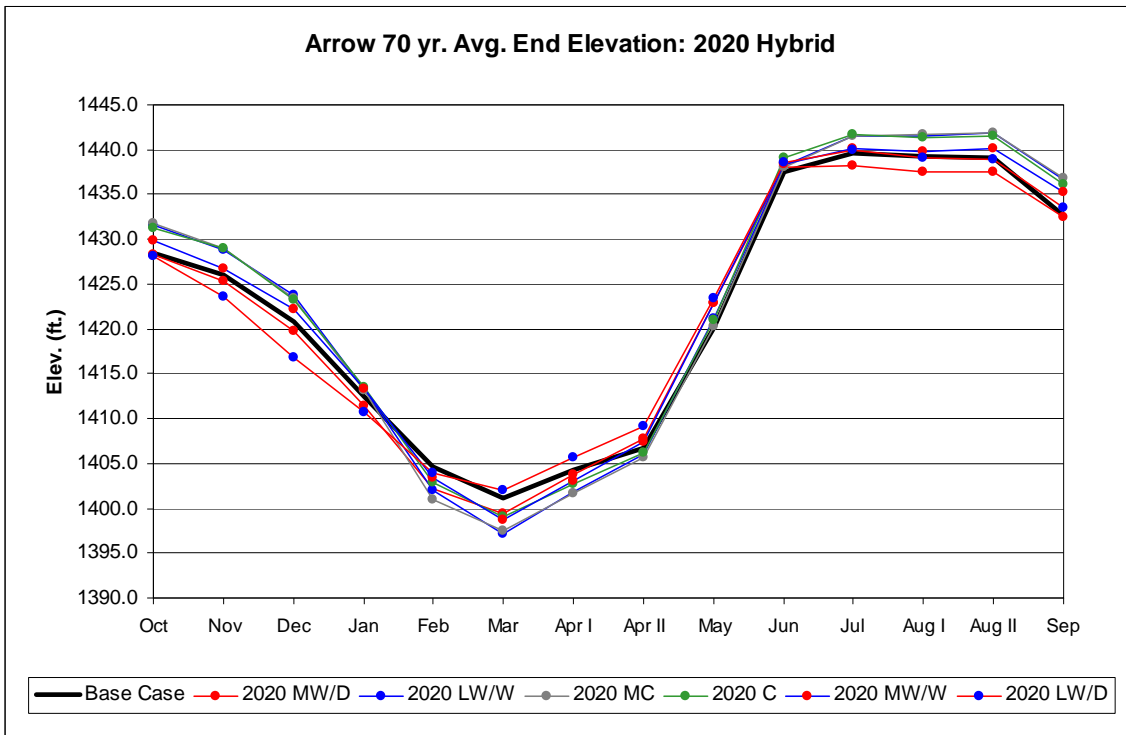
Figure 77. Arrow End Elevations: 2020s Hybrid-Delta.
