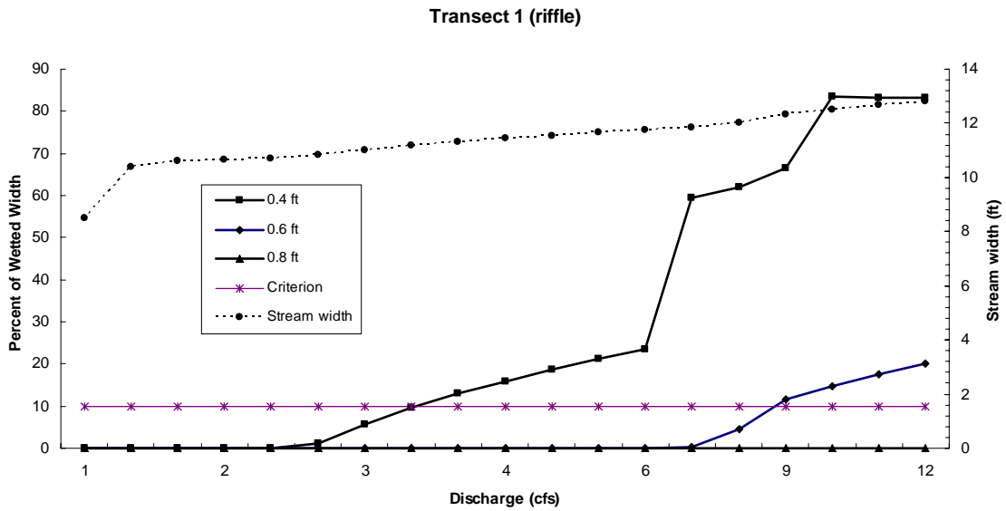
Figure 61. Contiguous widths at depths greater than passage criteria at a riffle transect on Bohannon Creek, Study Site 4.
