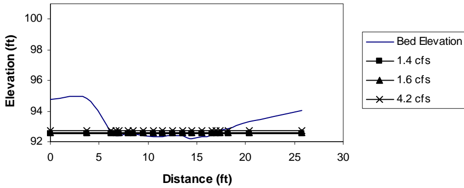
Transect 2
