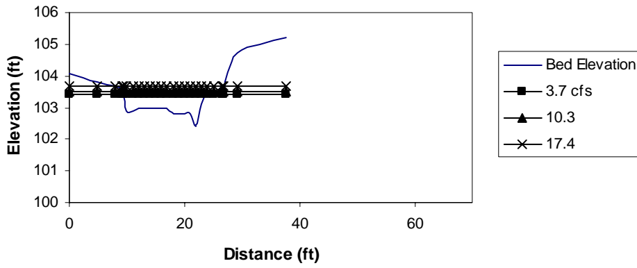
Transect 6
