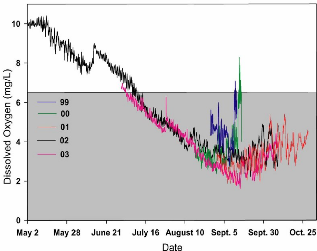
Figure 18. Seasonal Patterns of Decline in Dissolved Oxygen in the Canyon Ferry Tailrace as Measured at Riverside Campground. The gray area represents levels below the Montana Standard for Flowing Waters of 6.5 mg/L (Reclamation, 2004 - Figure 47).
