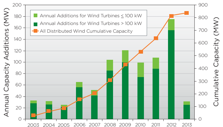
U.S. Distributed Wind Capacity
