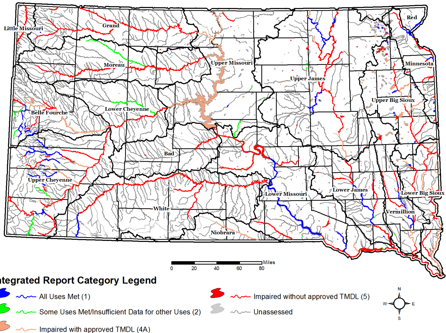
Figure 7: 2016 South Dakota Waterbody Status
