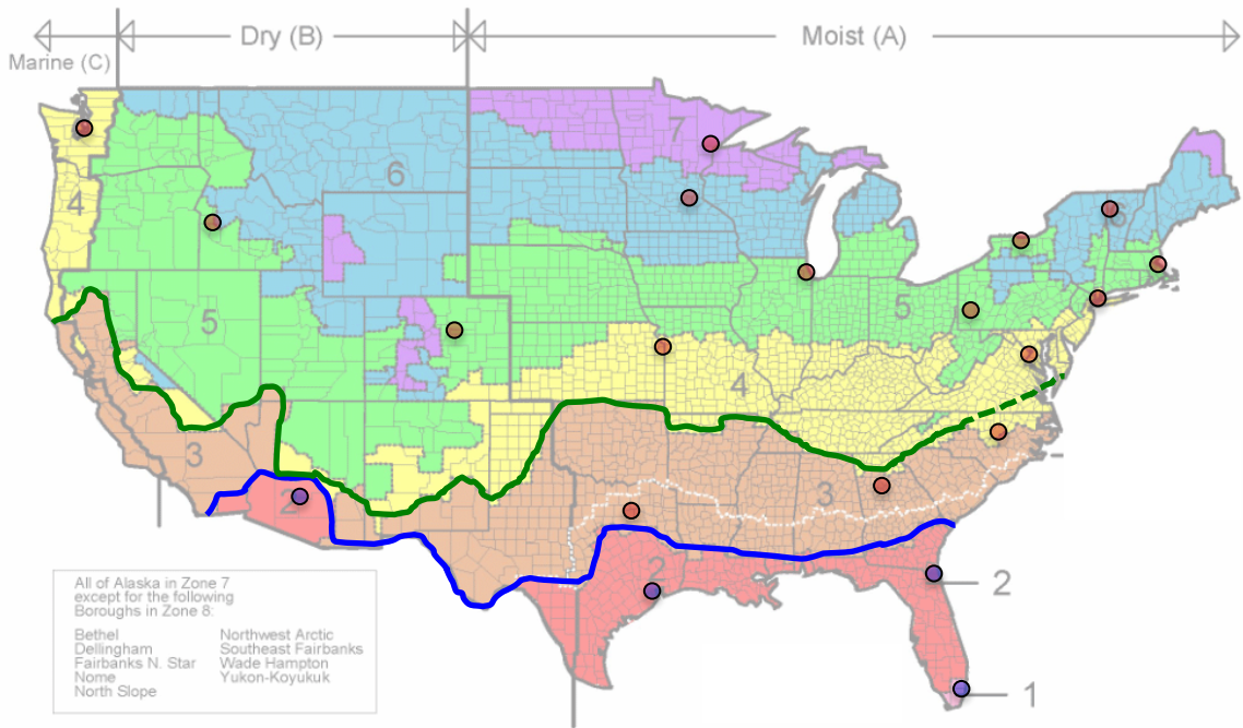
Figure 4.1 is a map with the overall general recommended regions for the use of low-e storm windows installed over single-pane windows and double-pane, metal-framed windows.
