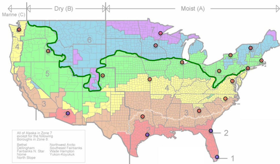
Figure 4.2 is a map with the overall general recommended regions for the use of low-e storm windows installed over double-pane, wood/vinyl-framed windows.
