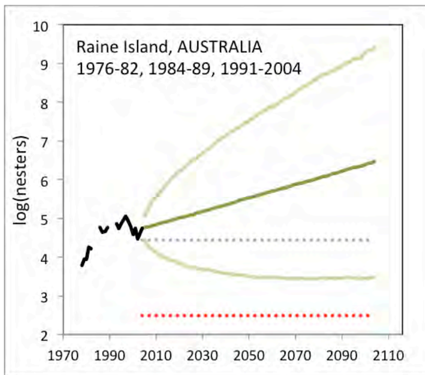
Figure 12.2. Stochastic Exponential Growth (SEG) Model Output for Raine Island, Australia. Black line is observed data, dark green line is the average of 10,000 simulations, green lines are the 2.5th and 97.5th percentiles, gray-green dotted line is trend reference, and red dotted line is absolute abundance reference. The units for the Raine Island indices are expressed as adult females, so no transformation from nests to nesters was needed.
