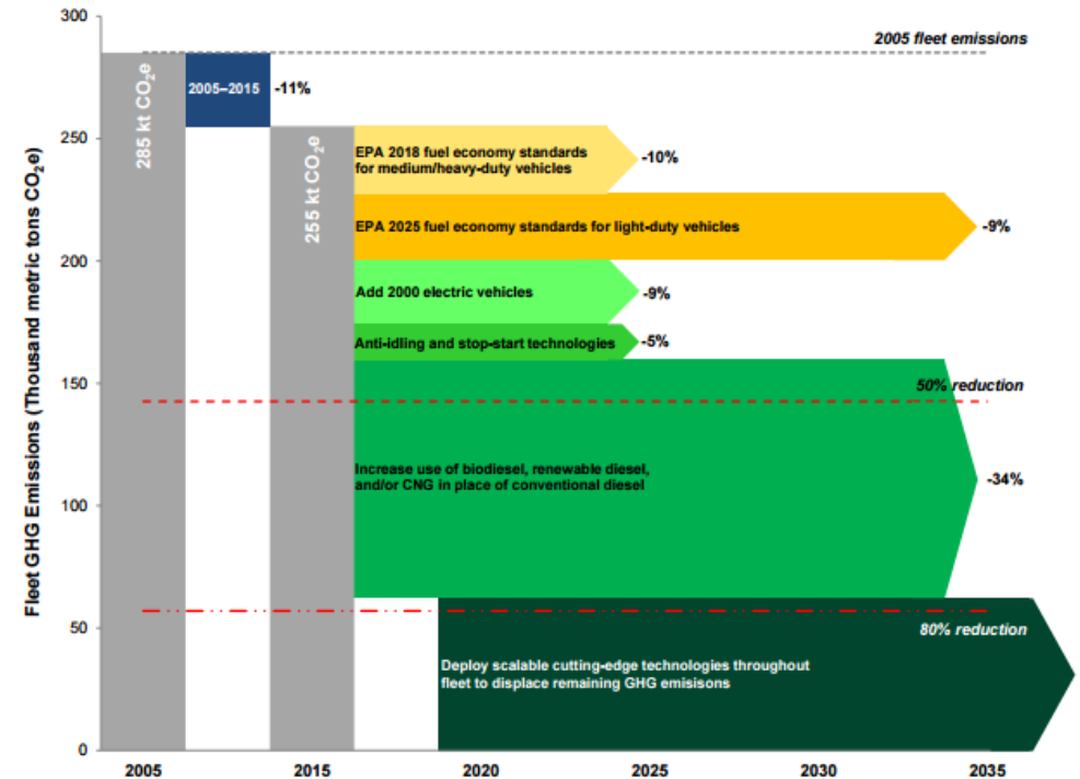
PATHWAYS TOWARD GHG EMISSIONS REDUCTIONS FOR NYC'S VEHICLE FLEET
