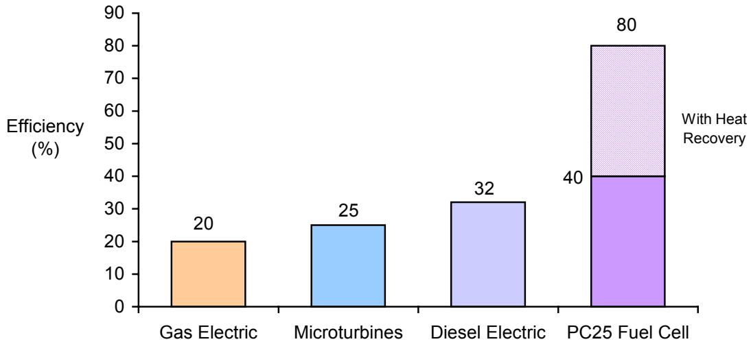
Figure 5. Phosphoric Acid Fuel Cell Efficiency Comparison
