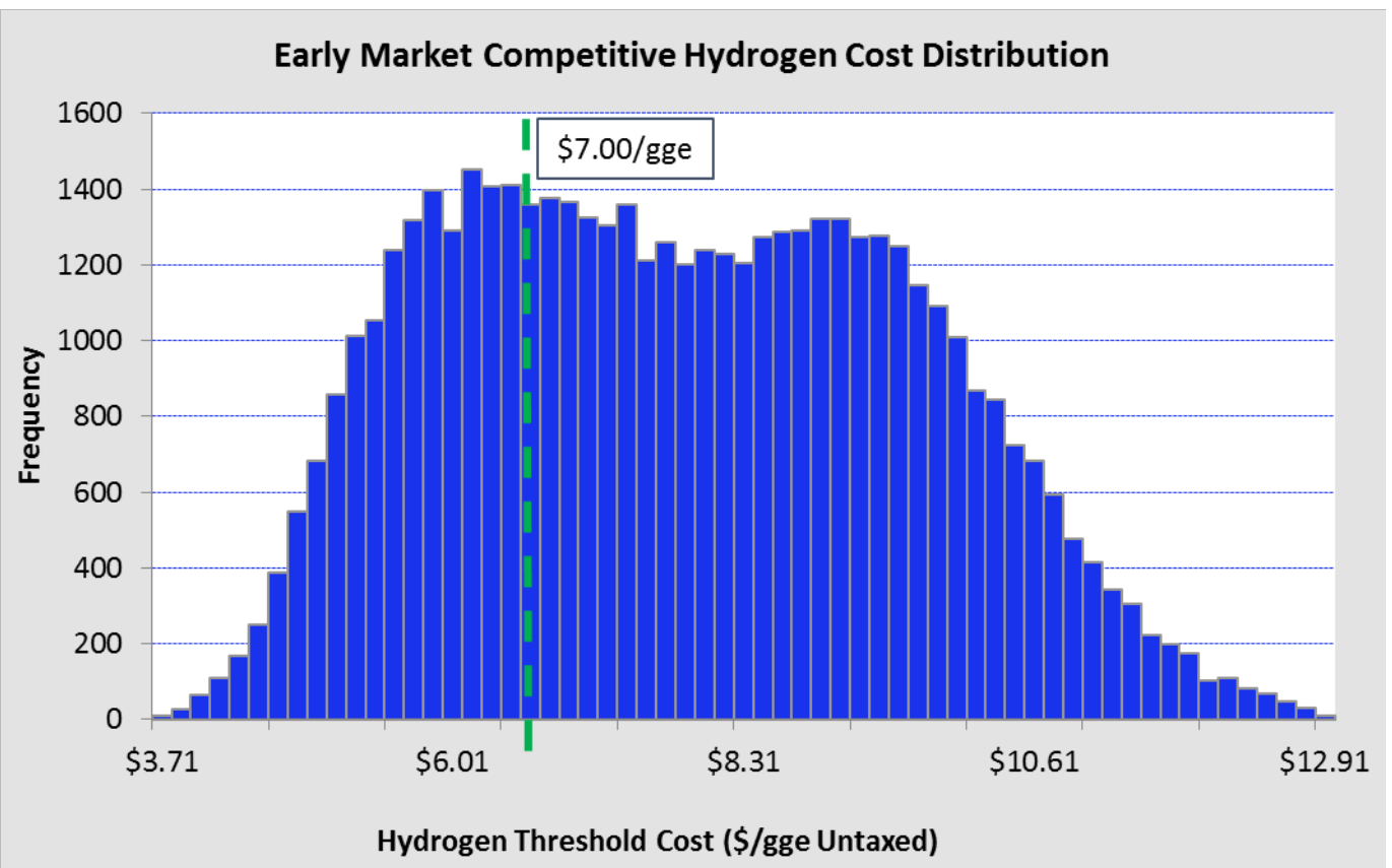
Figure 3: Histogram of Stochastic Analysis Results for Competitive Hydrogen Costs
