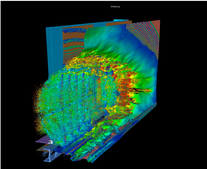
A 32,768 CTH simulation helps designers understand the response structures under severe blast loading conditions so that the robustness of these structures may be improved. A structure composed of sheet metal is loaded by an explosive blast. The plot gives the velocities of various components of the structure as they are torn apart. Accurately resolving these thin parts required a very fine mesh resolution which can presently be achieved using only very large scale computing platforms. (SNL)
