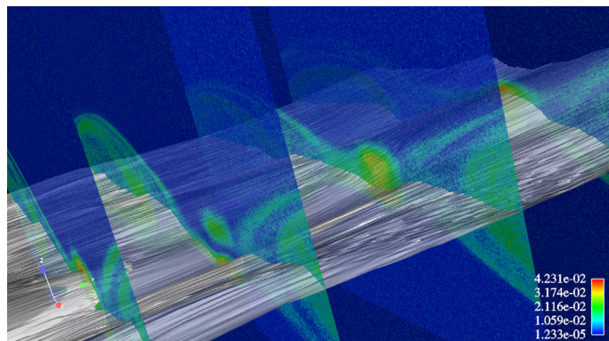
Magnetic islands and drift-kink instability observed in 3D large-scale fully kinetic VPIC simulations run on the Roadrunner base system of magnetic reconnection in electron-positron plasma. (LANL)
