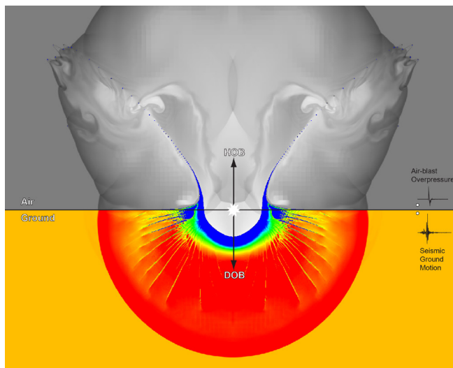
Monitoring of nuclear tests requires predictions of complex seismic wave propagation to differentiate earthquakes and explosions. (LLNL)
