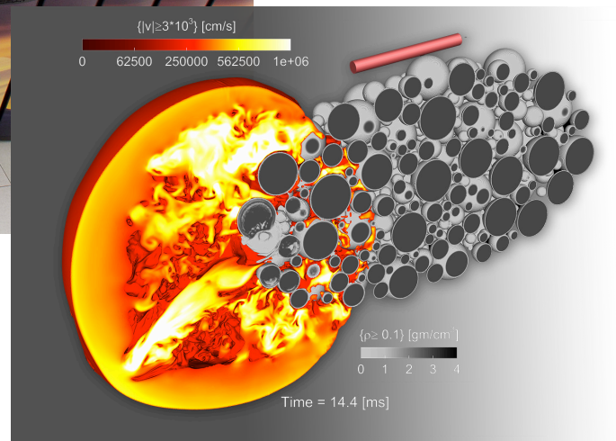
Astroid simulation: Full-physics, full-geometry, 3D simulation using 32,000 processors on Cielo to model a 500-kiloton nuclear blast to explode a 5-kilometer asteroid (Cielo/LANL)
