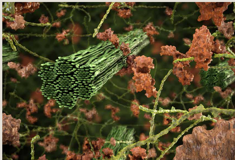
Fig. 3. Three-Dimensional Illustration of Lignocellulose Meshwork. Researchers are using computational modeling to gain a molecular-level understanding of the plant cell wall and its major components, including cellulose fibers (green), lignin molecules (brown wooden texture), and hemicellulose (light green). [Image courtesy Thomas Splettstoesser, www.scistyle.com , for Oak Ridge National Laboratory]
