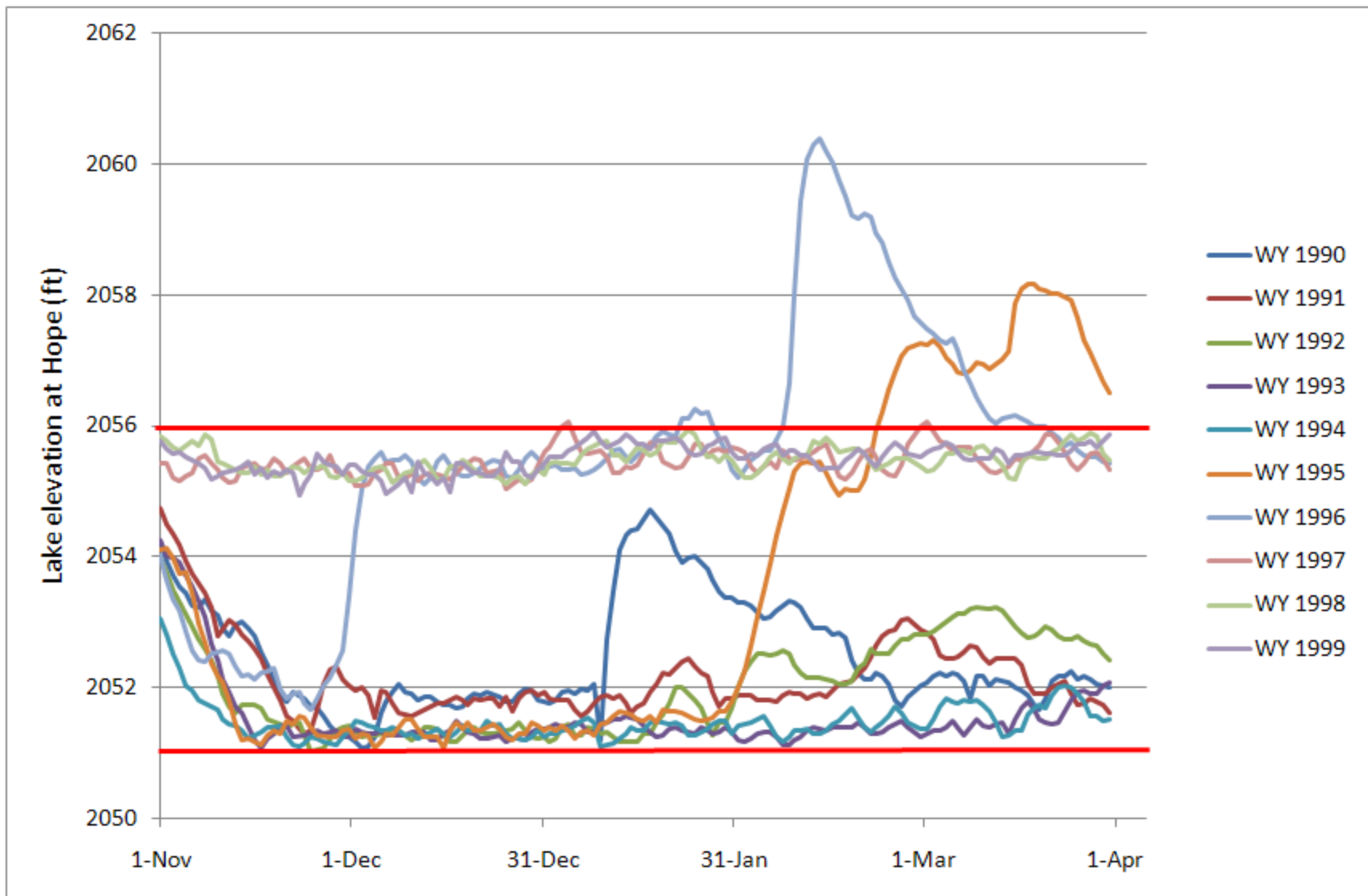
Figure B-4. Winter Elevation of Lake Pend Oreille, Water Years 1990–1999 (Water year is from October 1 to September 30. Red lines denote FWPO operating range.)
