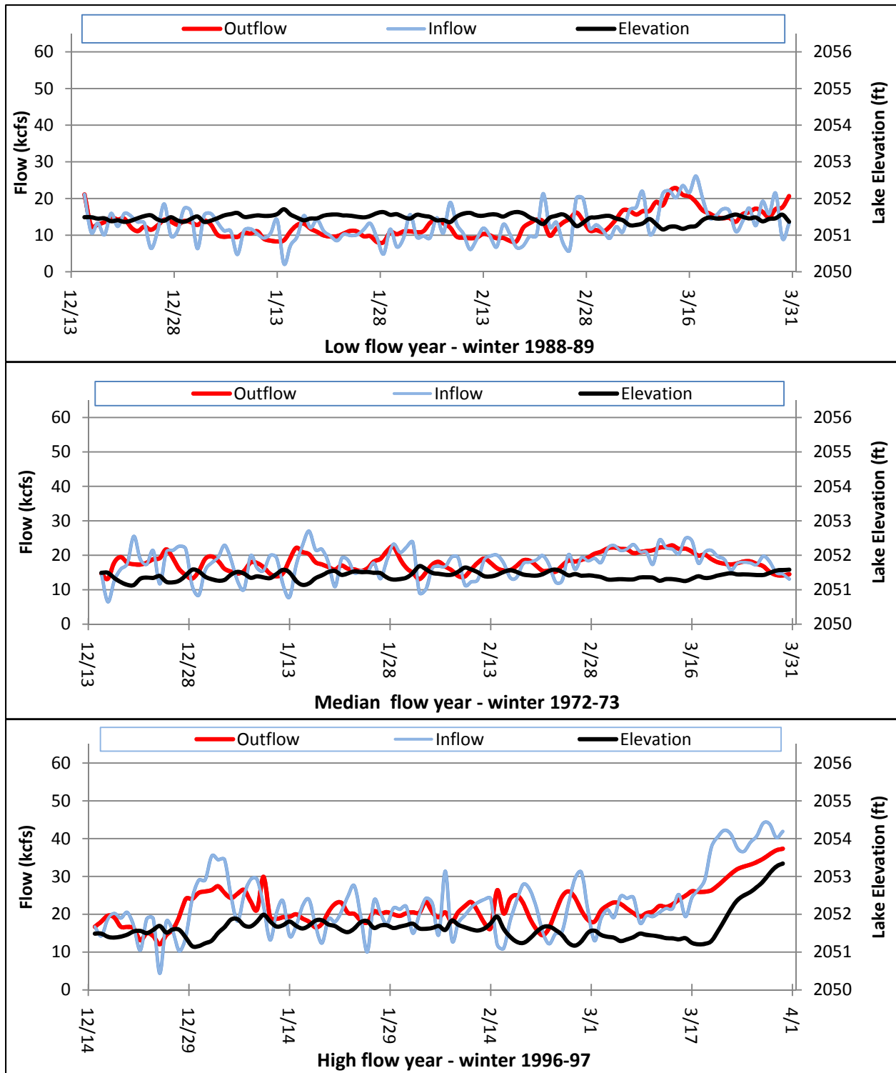
Figure 4-2. No Action Alternative Operations Inflow, Outflow, and Lake Elevation with MCE of 2051 feet for Low (10 th percentile), Median (50 th percentile), and High (90 th percentile) Flow Years.
