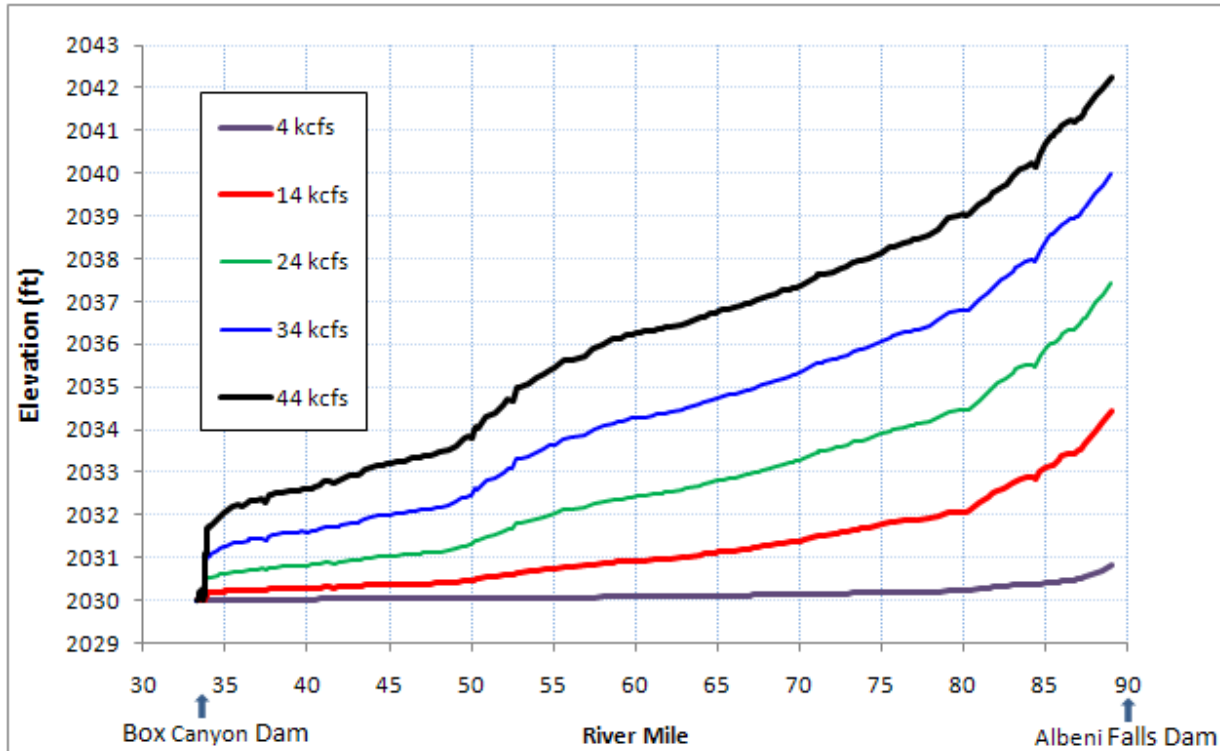
Figure 4-4. Modeled River Stage and Discharge (non-ice conditions) in the Pend Oreille River between Albeni Falls Dam and Box Canyon Dam for the Range of Flows Possible under FWPO (assumes BCD forebay = 2030 feet).
