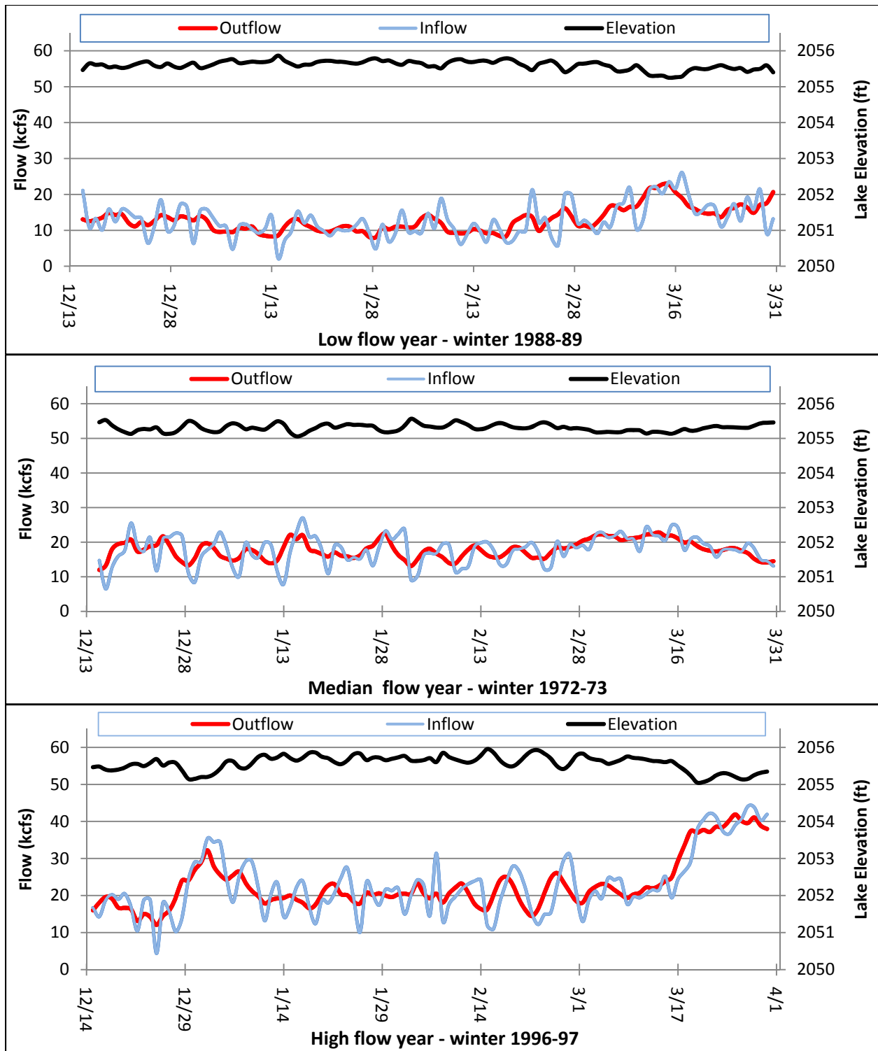
Figure 4-3. No Action Alternative Operations Inflow, Outflow, and Lake Elevation with MCE of 2055 feet for Low (10 th percentile), Median (50 th percentile), and High (90 th percentile) Flow Years.
