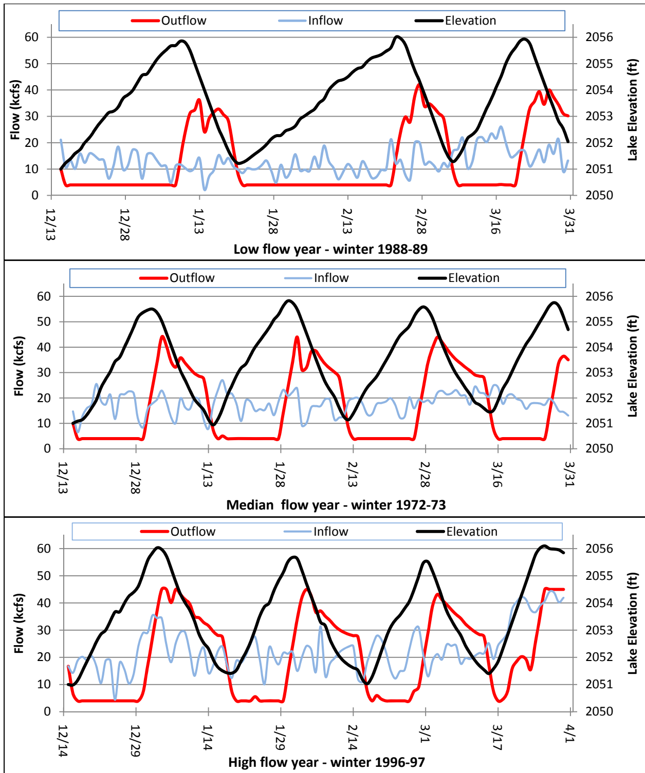
Figure 4-1. Flexible Winter Power Operations Inflow, Outflow, and Lake Elevation for Low (10 th percentile), Median (50 th percentile), and High (90 th percentile) Inflow Years.
