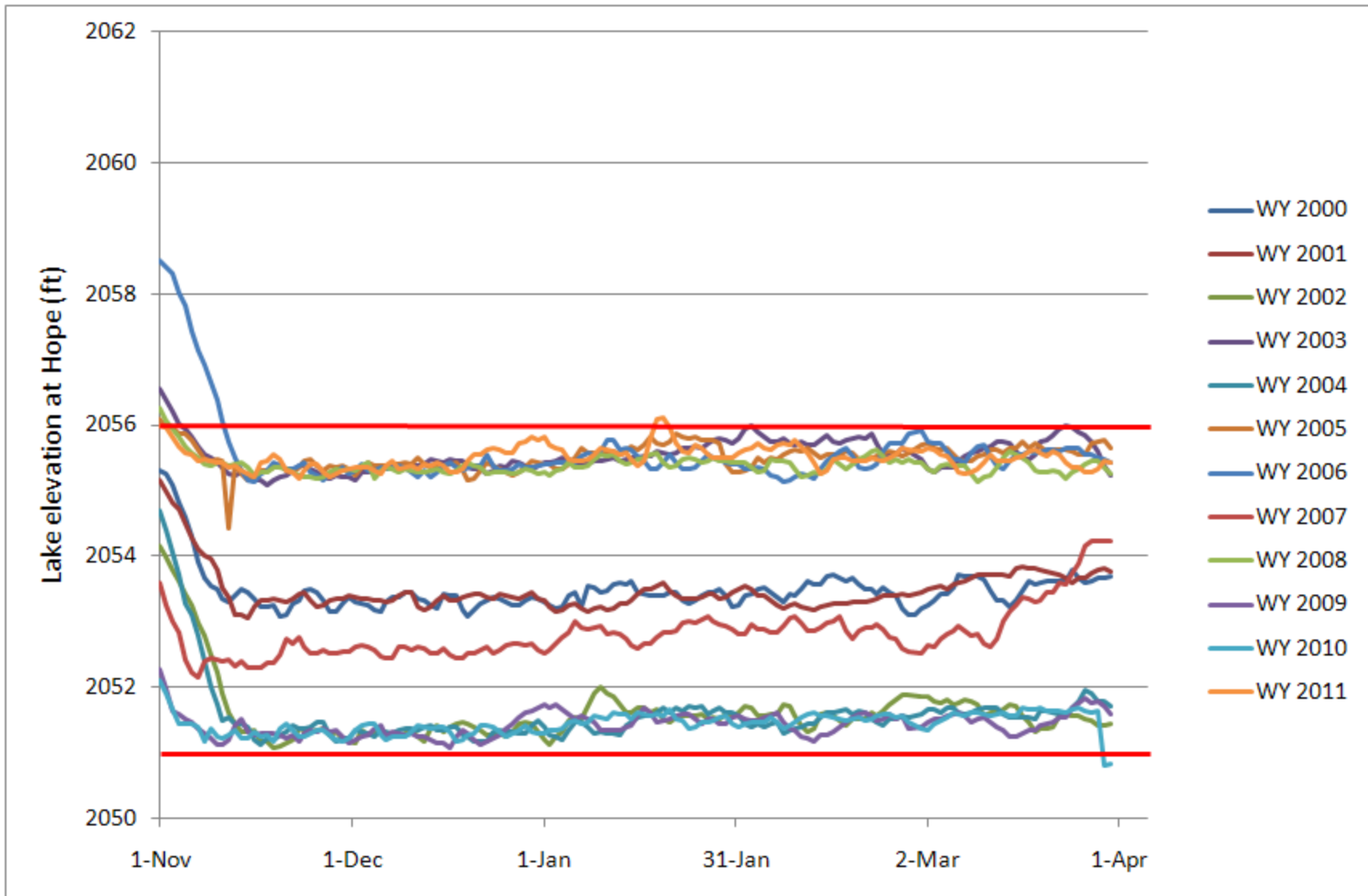
Figure B-5. Winter Elevation of Lake Pend Oreille, Water Years 2000–2011
