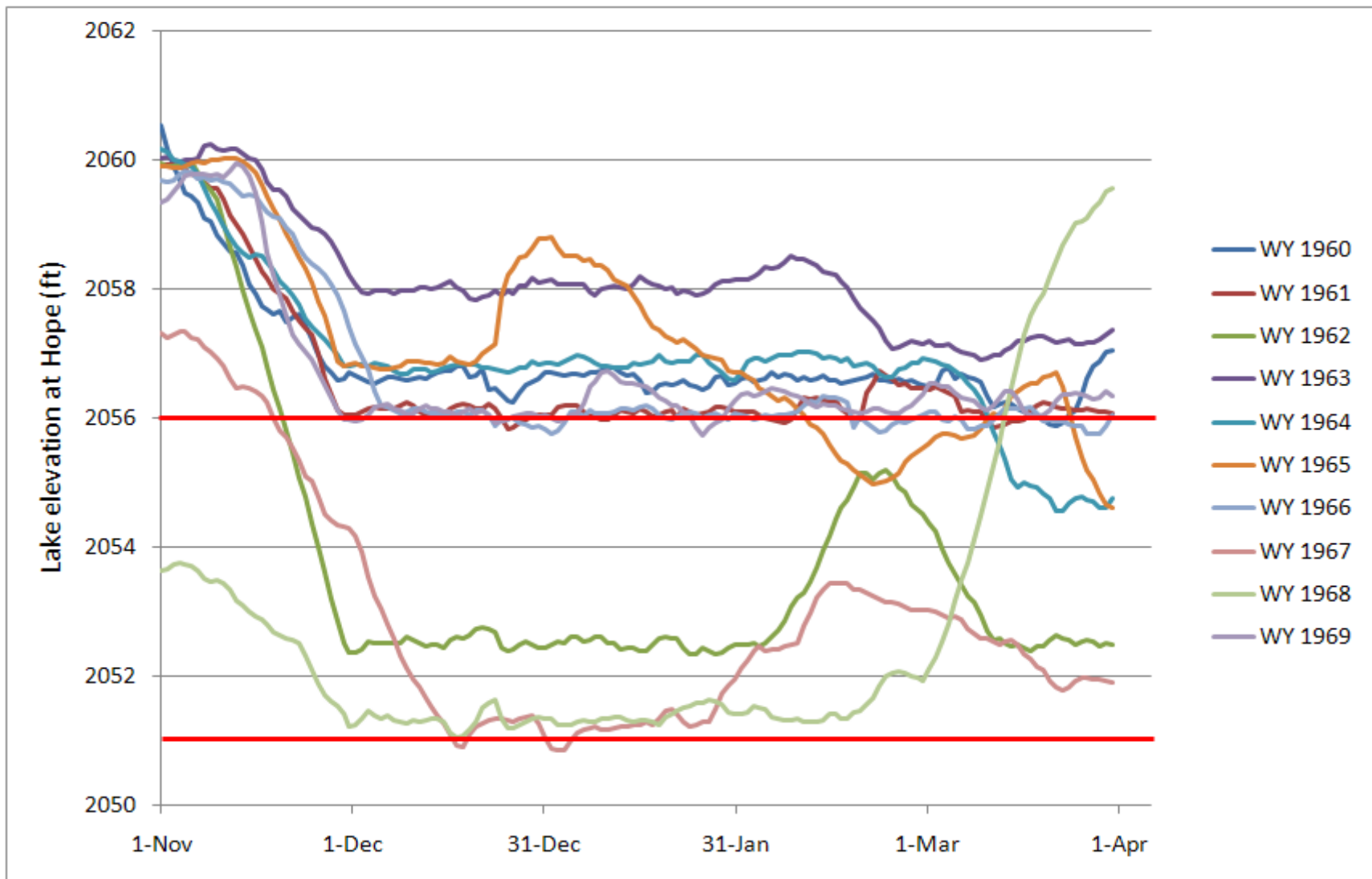
Figure B-1. Winter Elevation of Lake Pend Oreille, Water Years 1960–1969 (Water Year is from October 1 to September 30. Red lines denote the FWPO operating range.)
