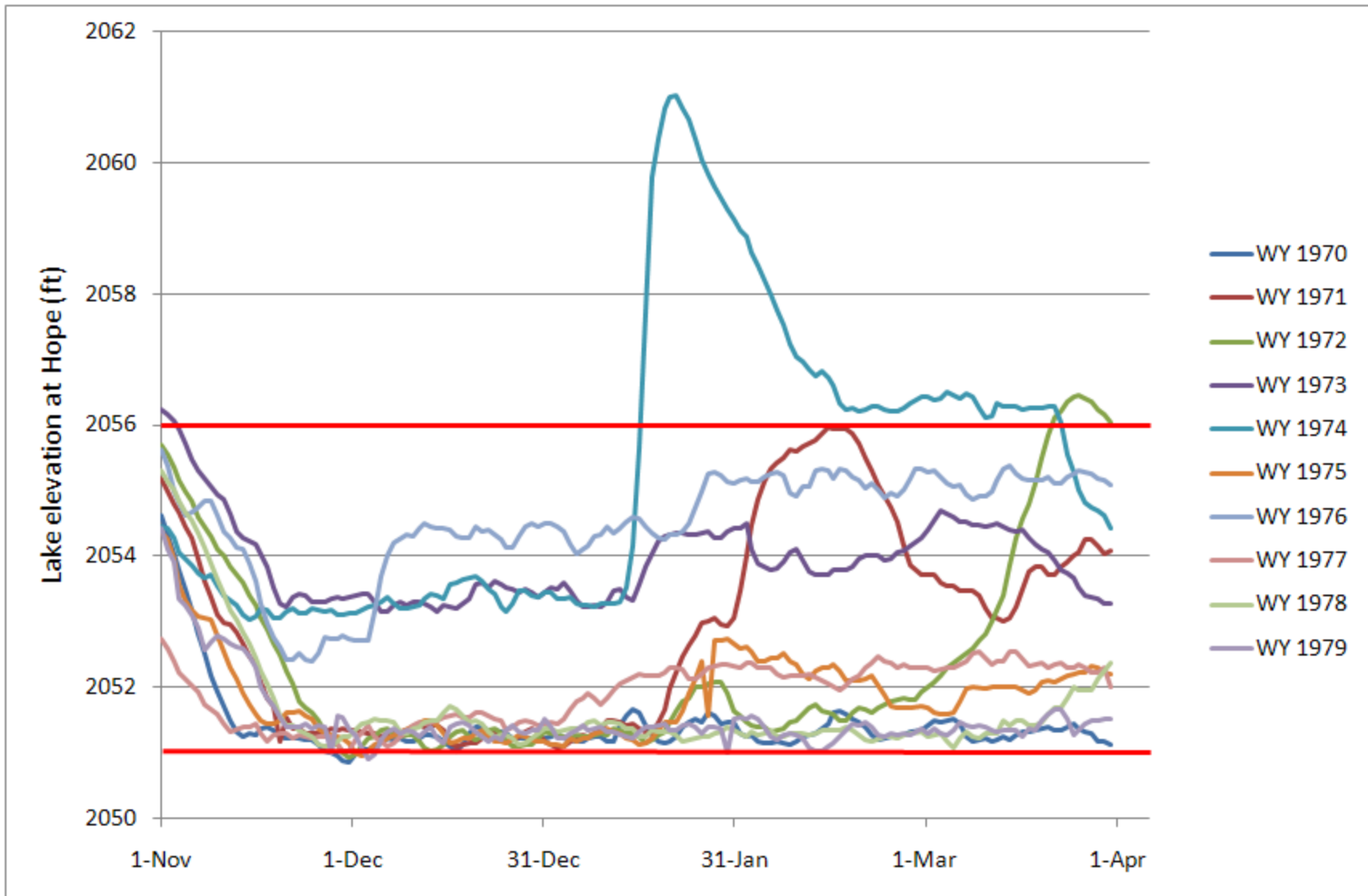
Figure B-2. Winter Elevation of Lake Pend Oreille, Water Years 1970–1979 (Water year is from October 1 to September 30. Red lines denote the FWPO operating range.)
