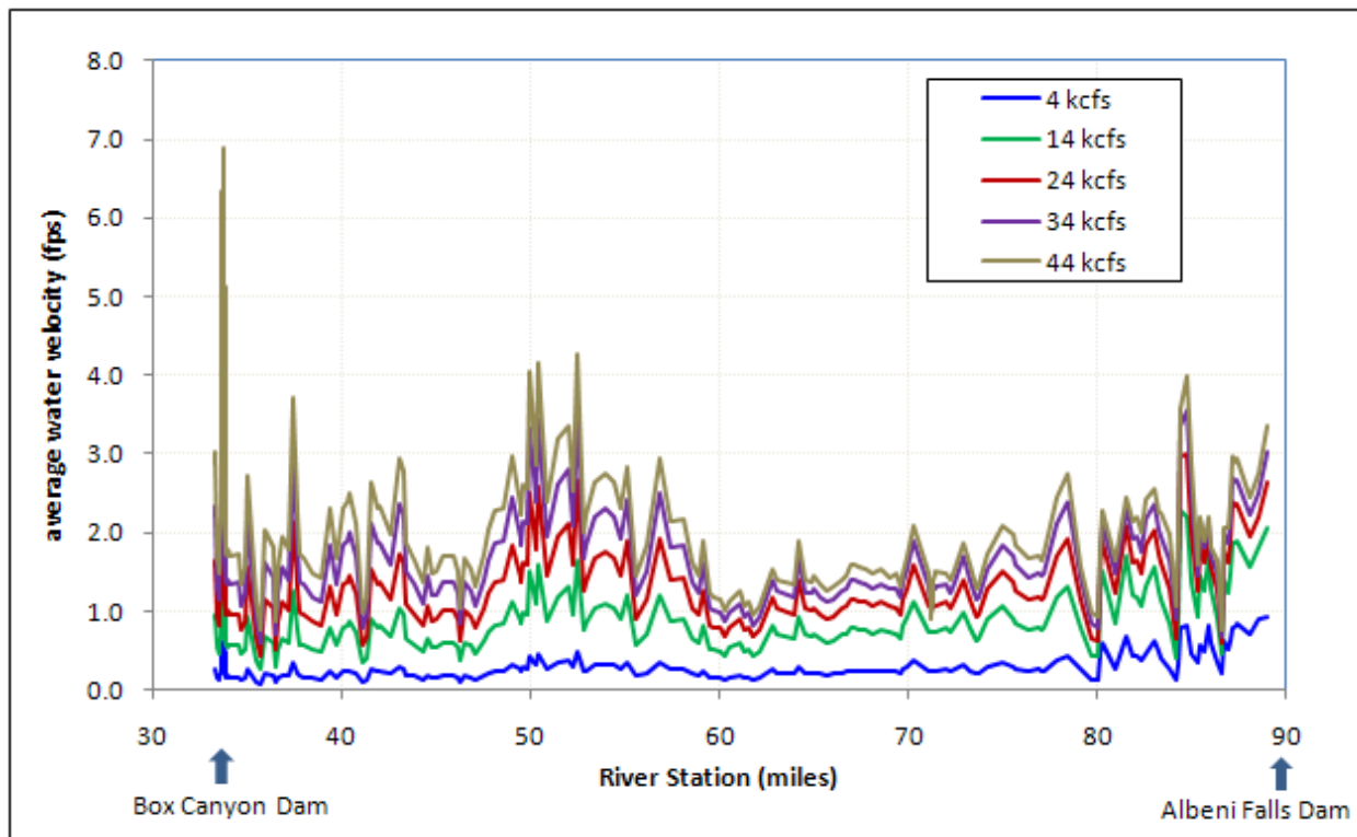
Figure 4-5. Average Modeled Water Velocity (non-ice conditions) in the Pend Oreille River between Albeni Falls Dam and Box Canyon Dam for the Range of Flows under FWPO. Velocity is slightly less for ice cover conditions.
