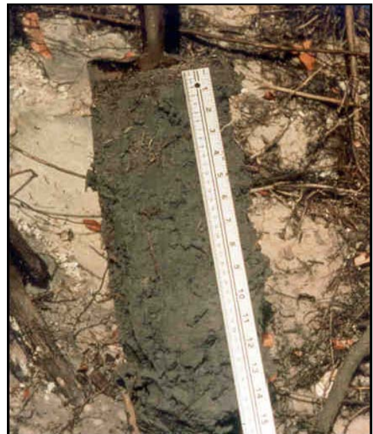
Figure 11. In this example, the gleyed matrix begins at the soil surface.
