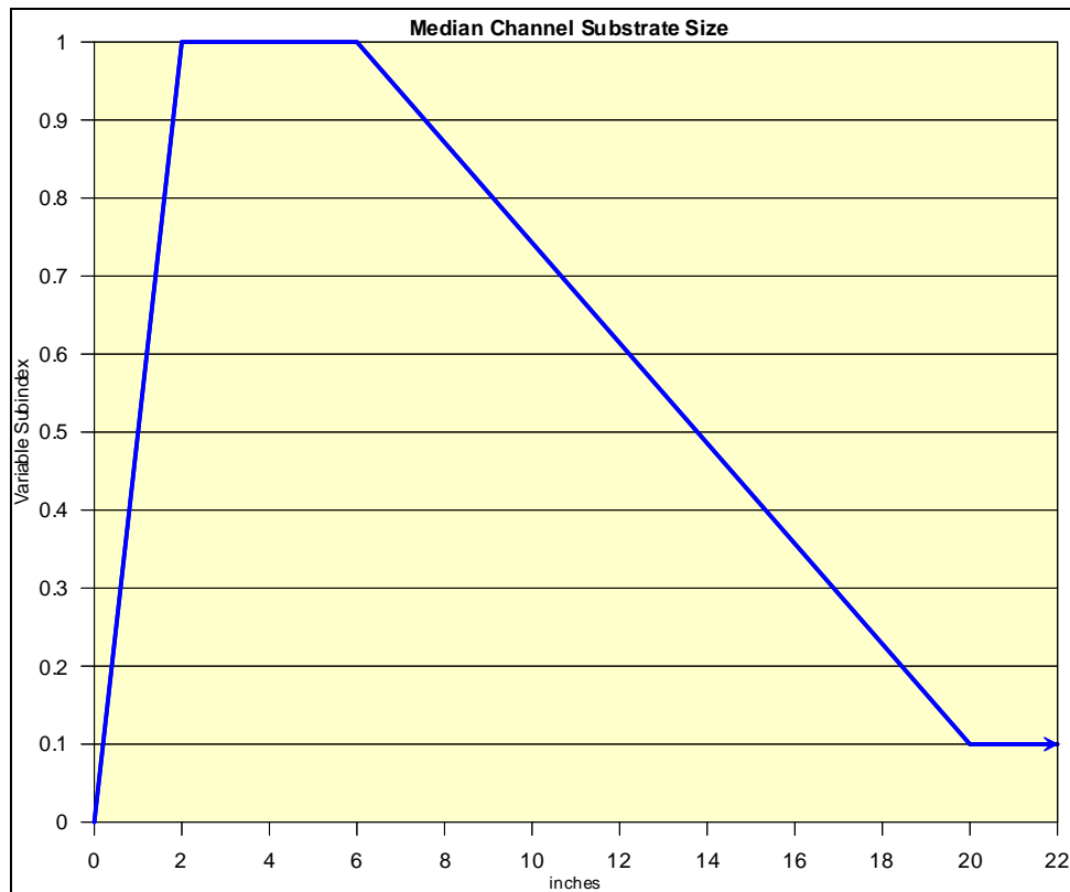
Figure 13. Relationship between median channel substrate size ( V_{SUBSTRATE} ) and functional capacity.
