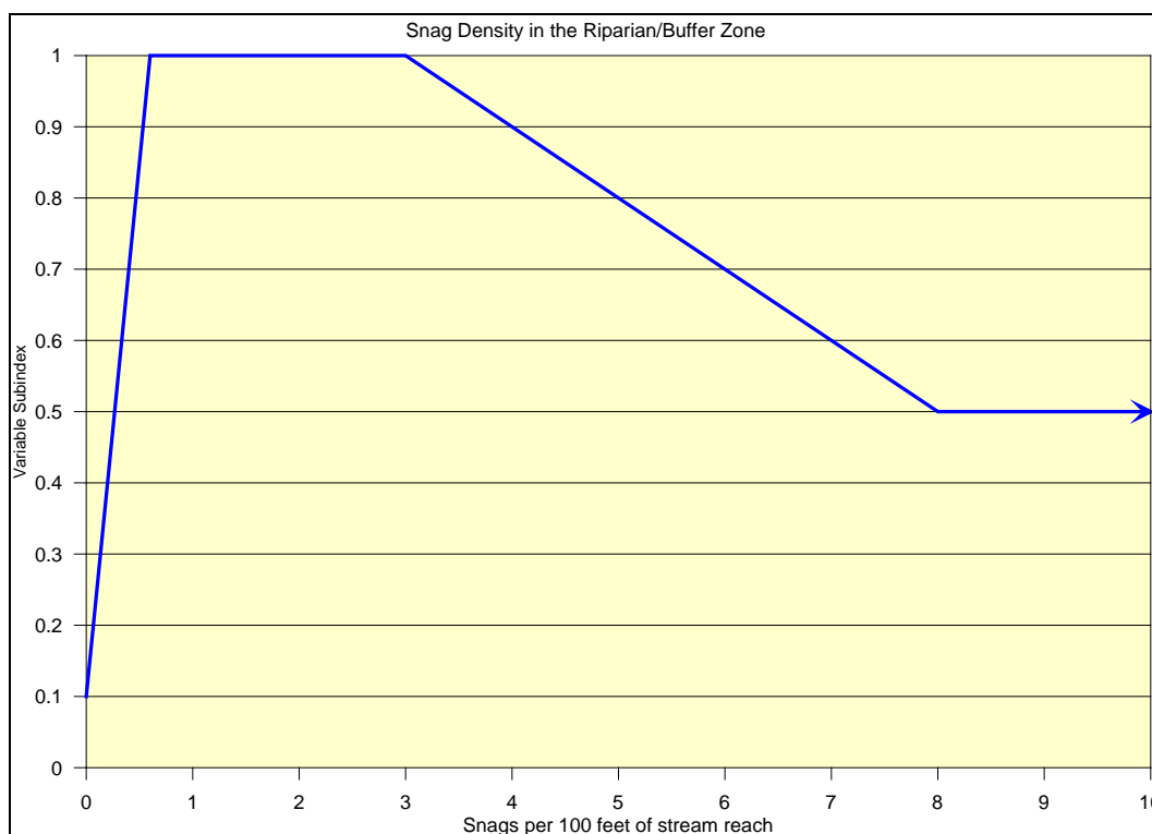
Figure 21. Relationship between density of snags in the riparian/buffer zone ( V_{SNA} ) and functional capacity.
