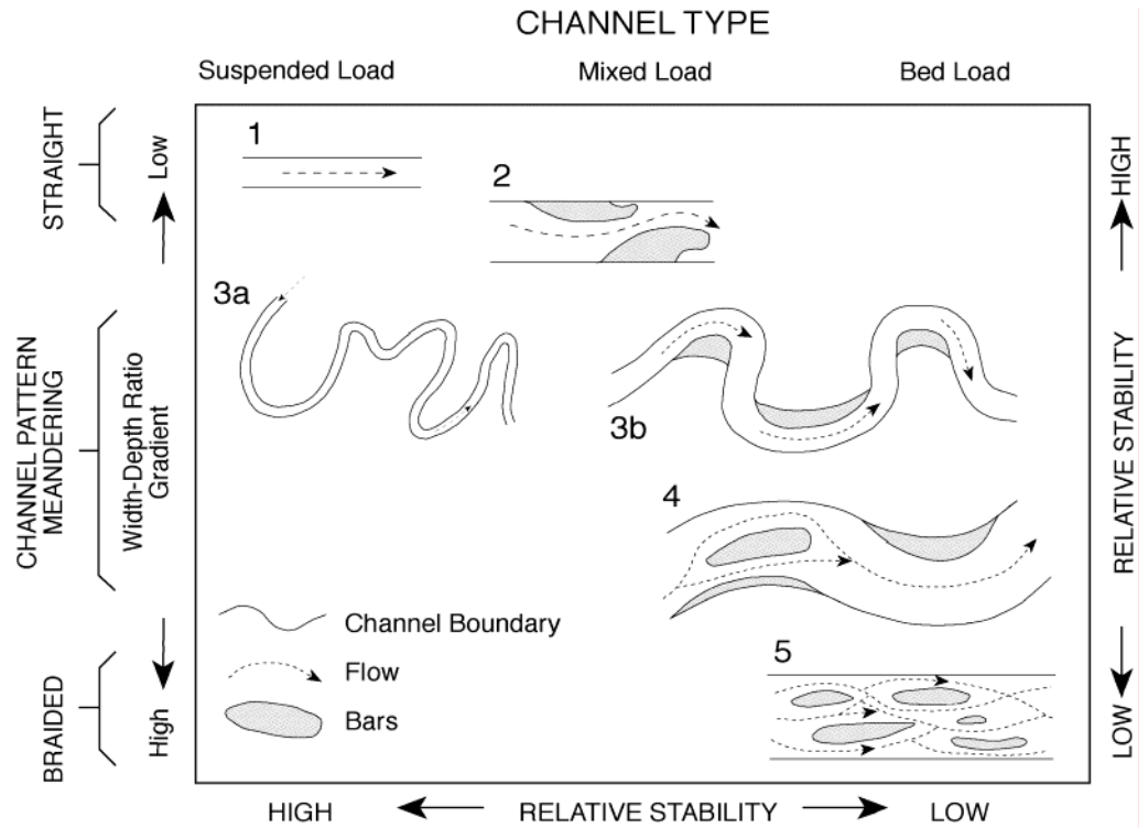
Figure 3.3 Classification of channel pattern based on sediment load and system stability (after Schumm, 1963).
